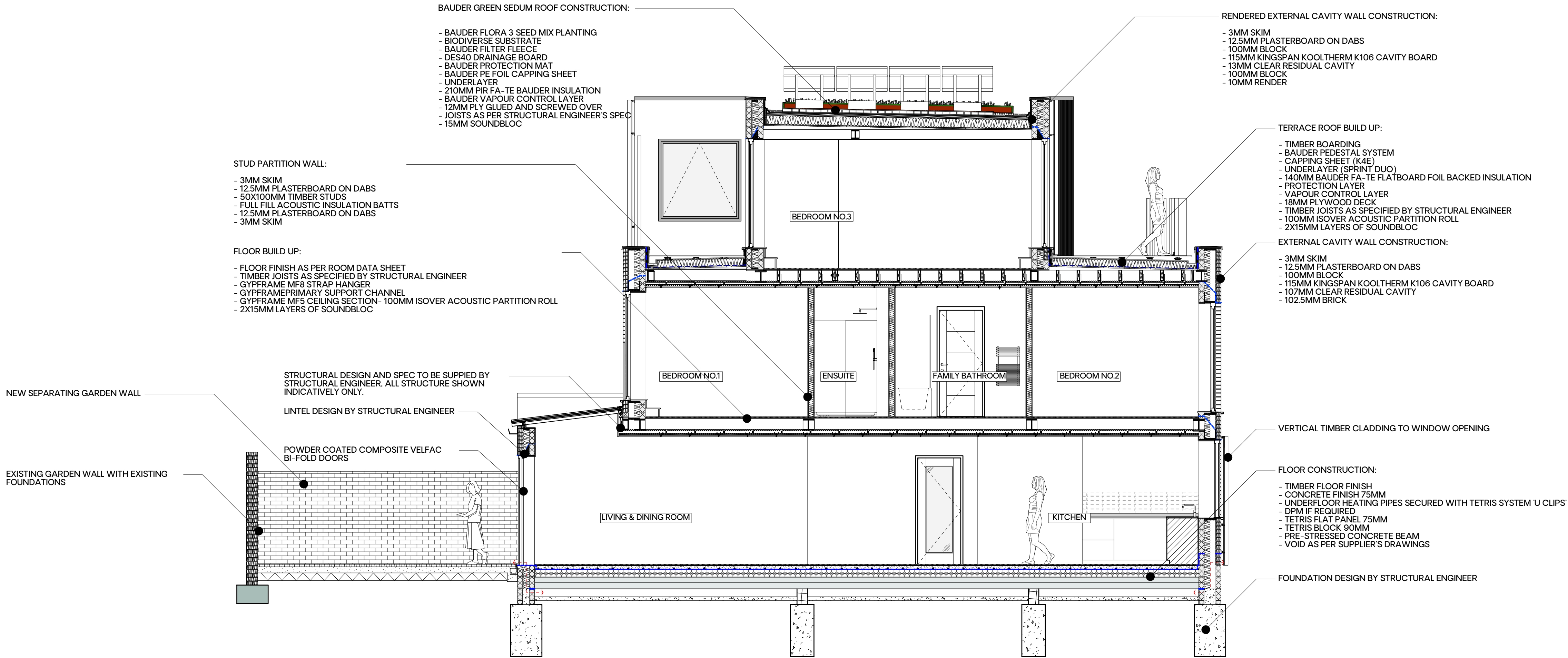
01 HOUSE C: PROPOSED SECTION 1:50 @ A1
