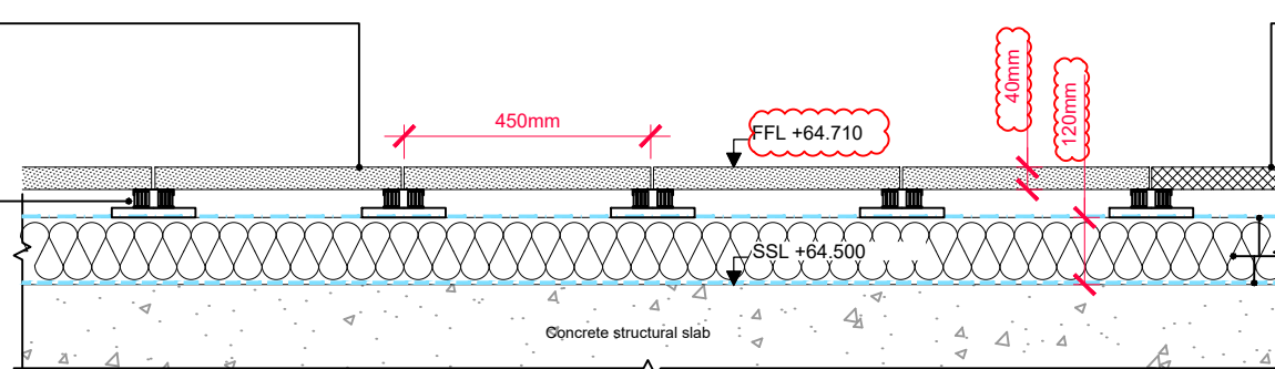
DETAIL 02: SECTION A-A' - LEVEL 10 PAVING TYPICAL DETAILED SECTION
