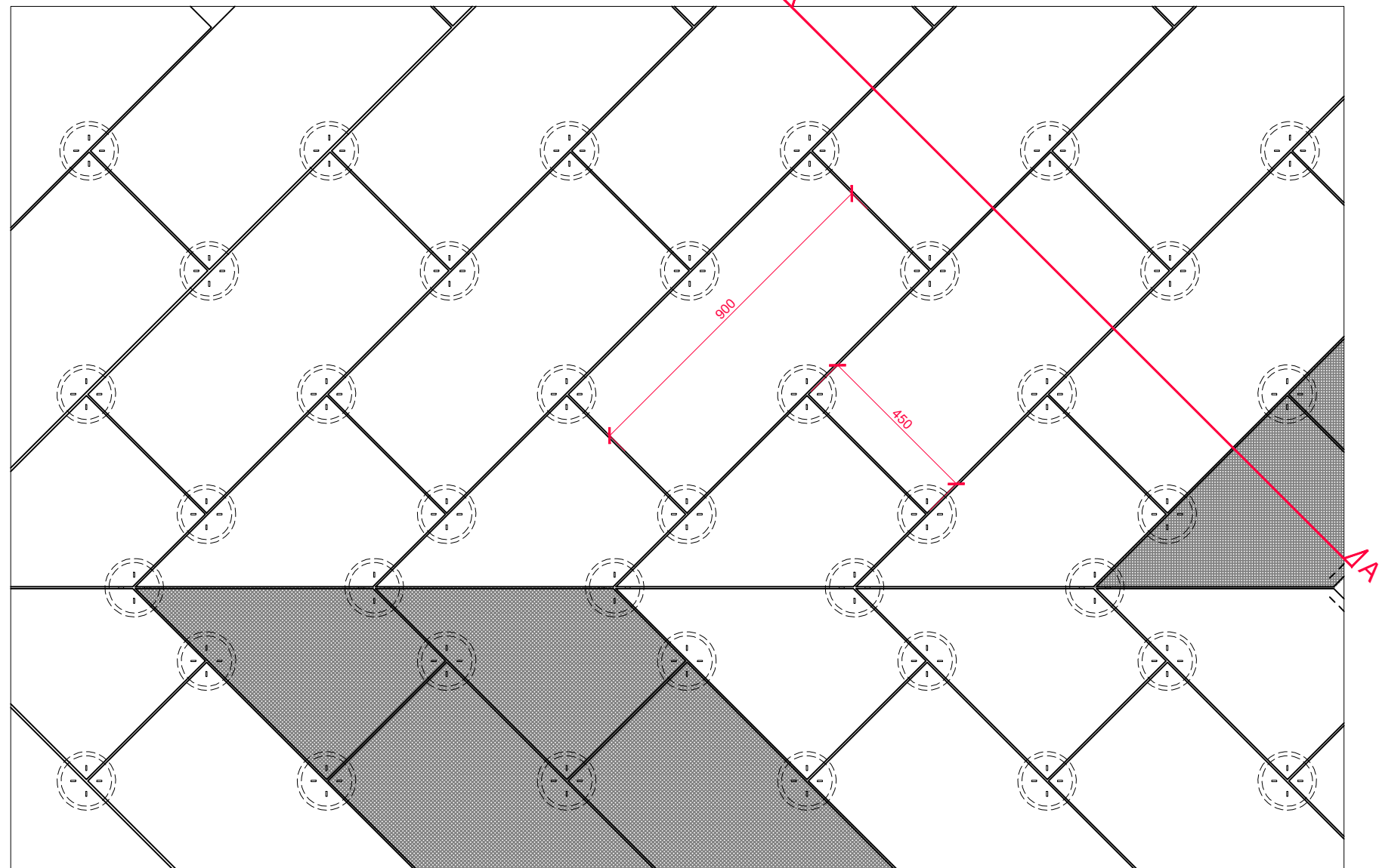
DETAIL 01: LEVEL 10 PAVING TYPICAL LAYOUT
