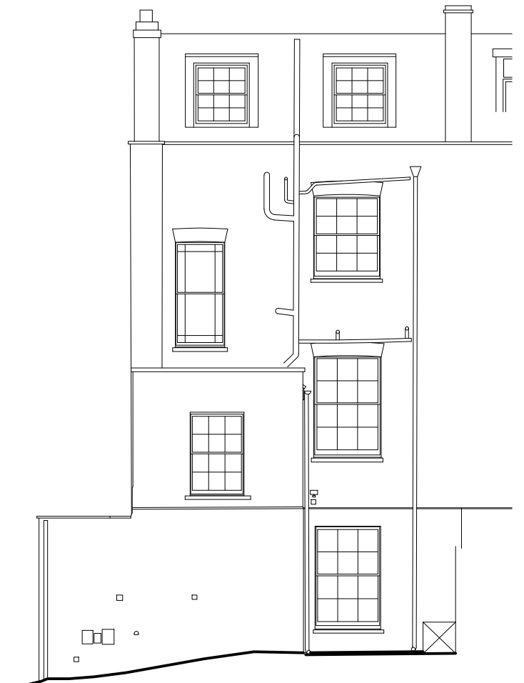
03 East Elevation 1200 1:100 @ A3
