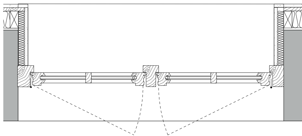
WINDOW TYPE 01: REPLACEMENT DOUBLE CASEMENT TOP AND SIDE HUNG OPENABLE
