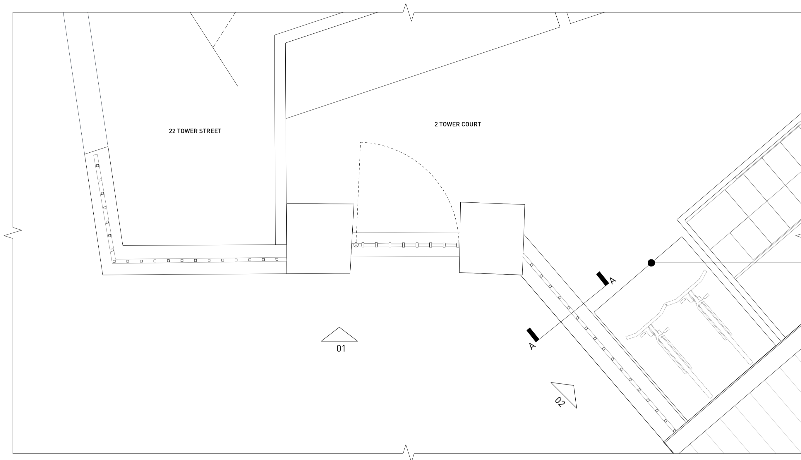
Plan 1:20 @ A1
