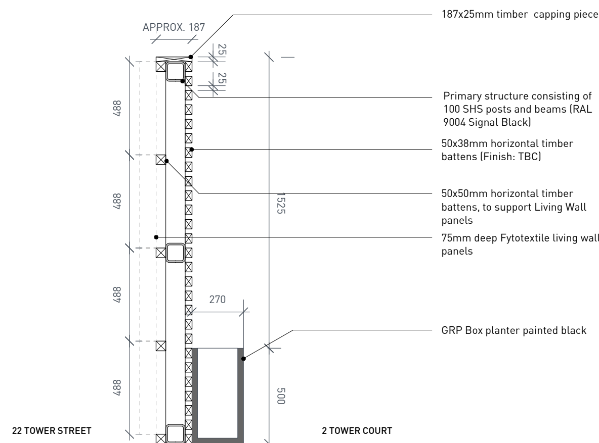
SECTION AA 1:20 @ A1
