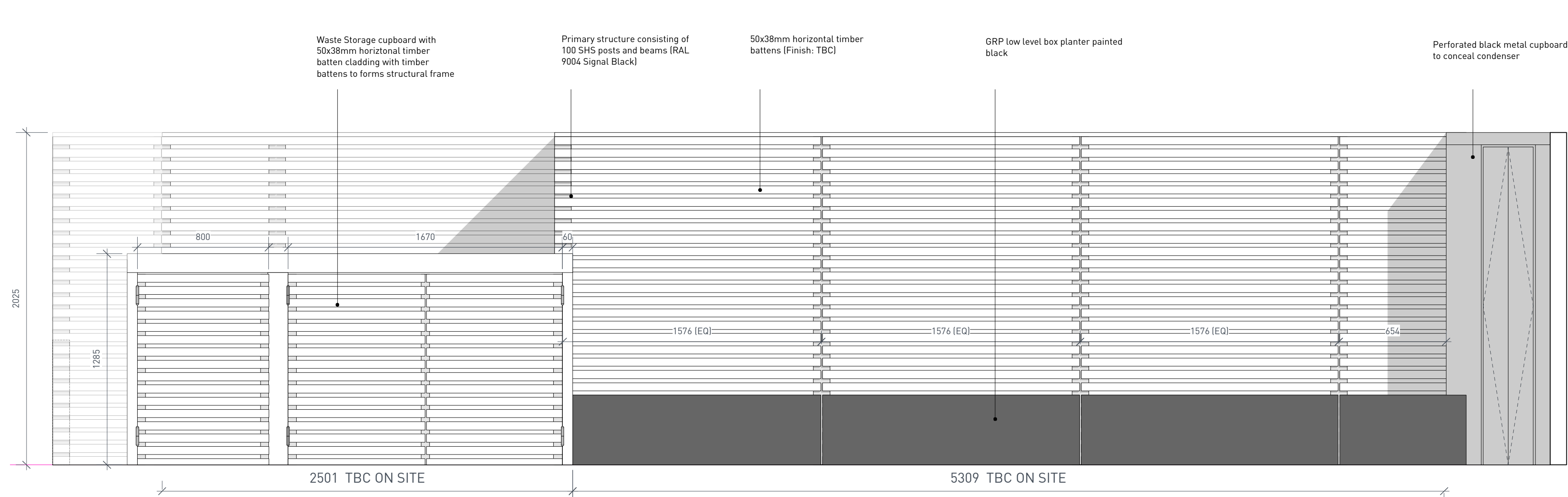
ELEVATION 01 1:20 @ A1
