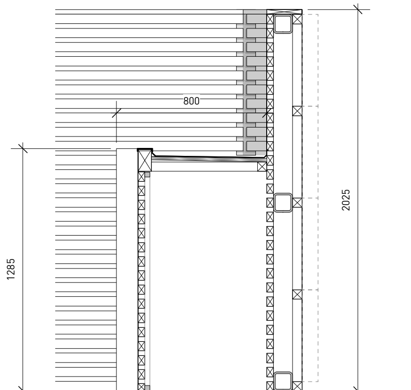
SECTION BB 1:20 @ A1
