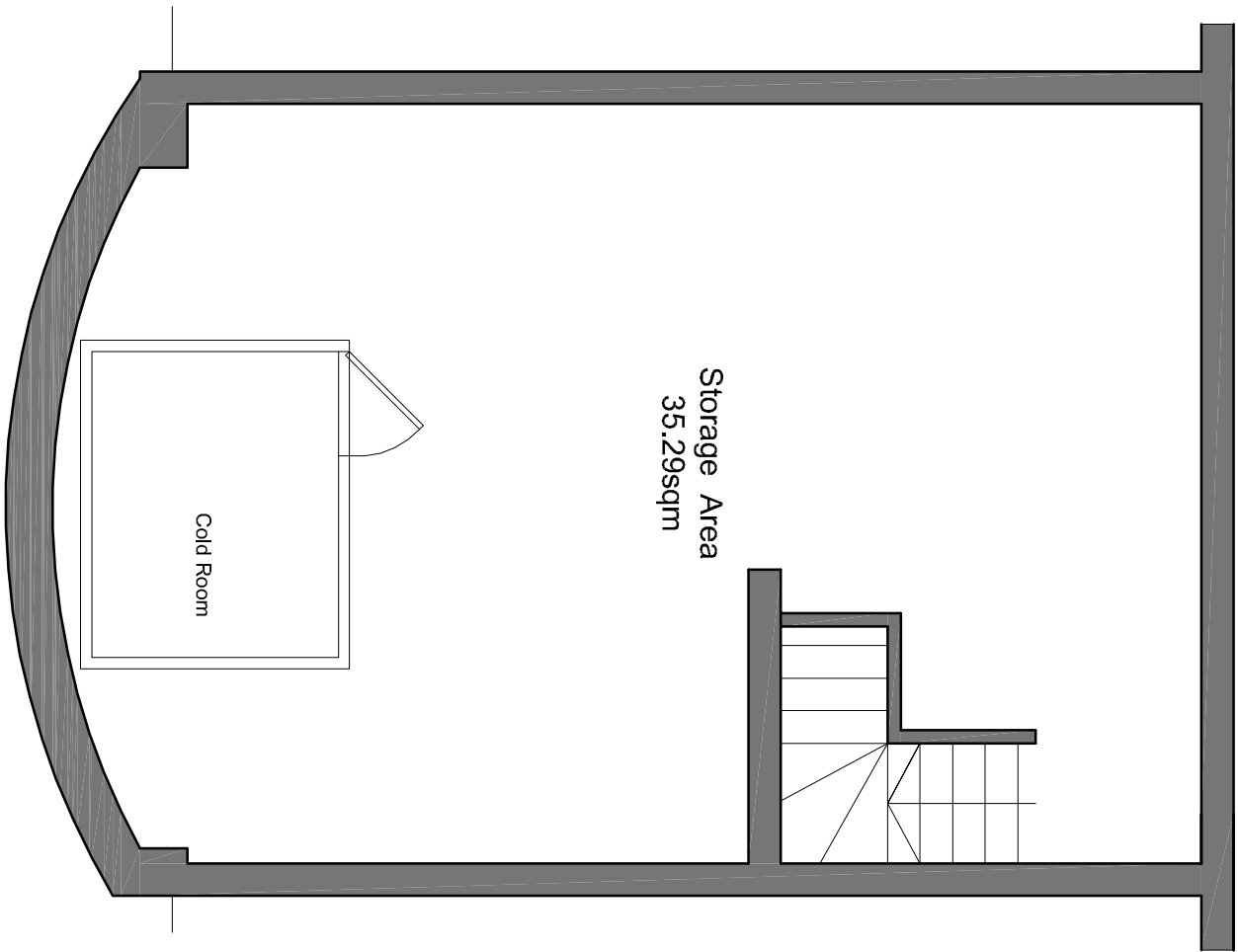
PROPOSED BASEMENT FLOOR PLAN
