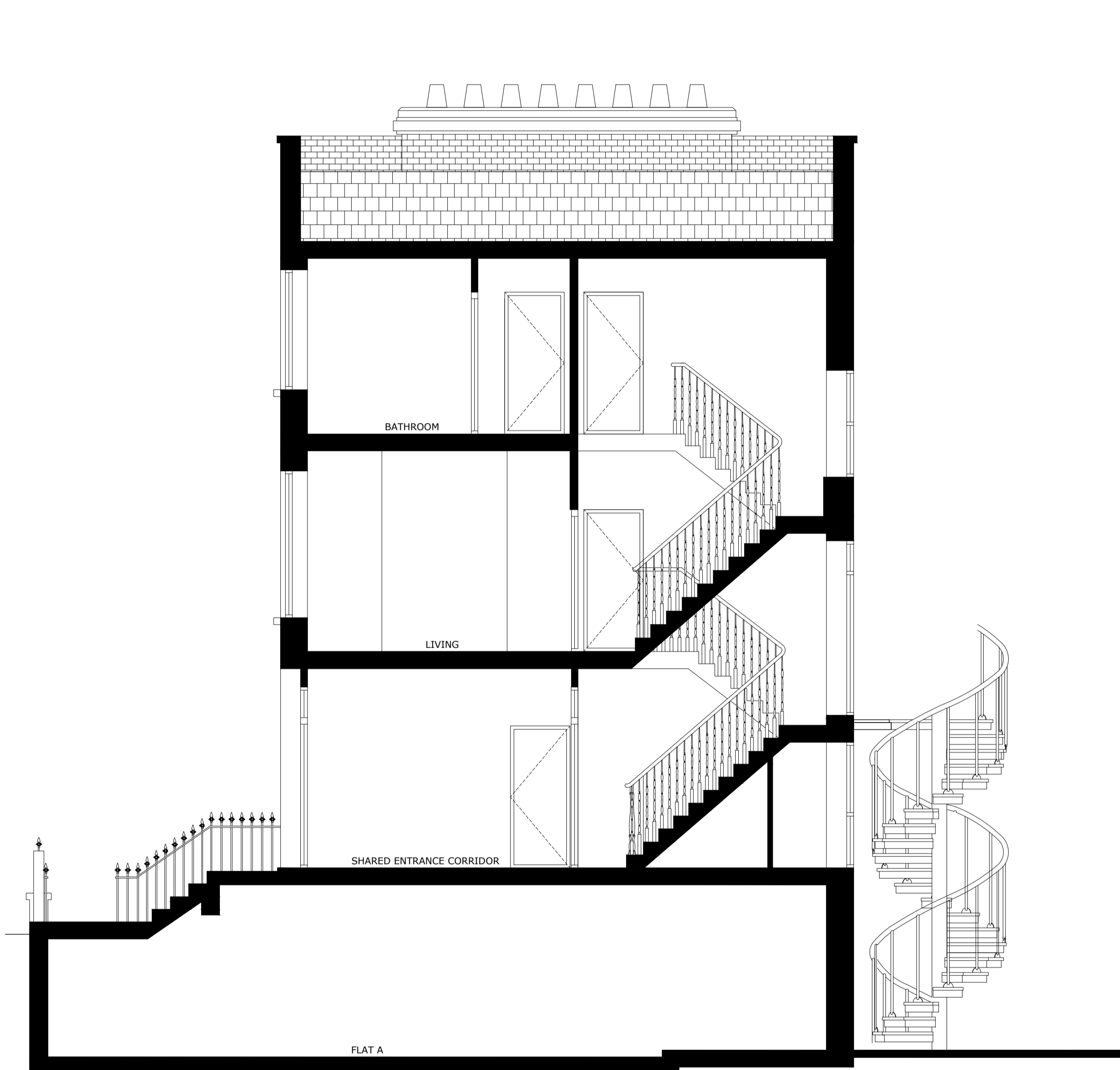
01 EXISTING SECTION AA 1:100 @ A3
