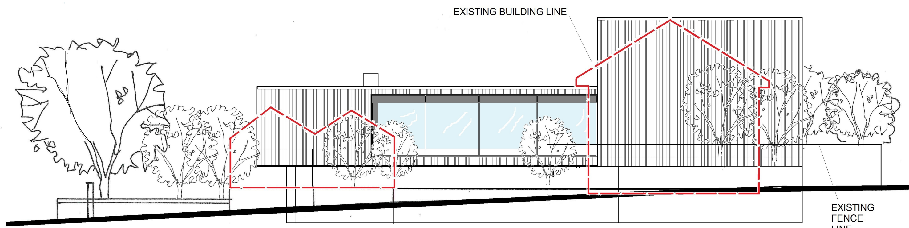
ELEVATON TO MILLFIELD PLACE
