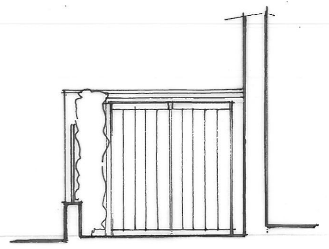
SECTION B-B
