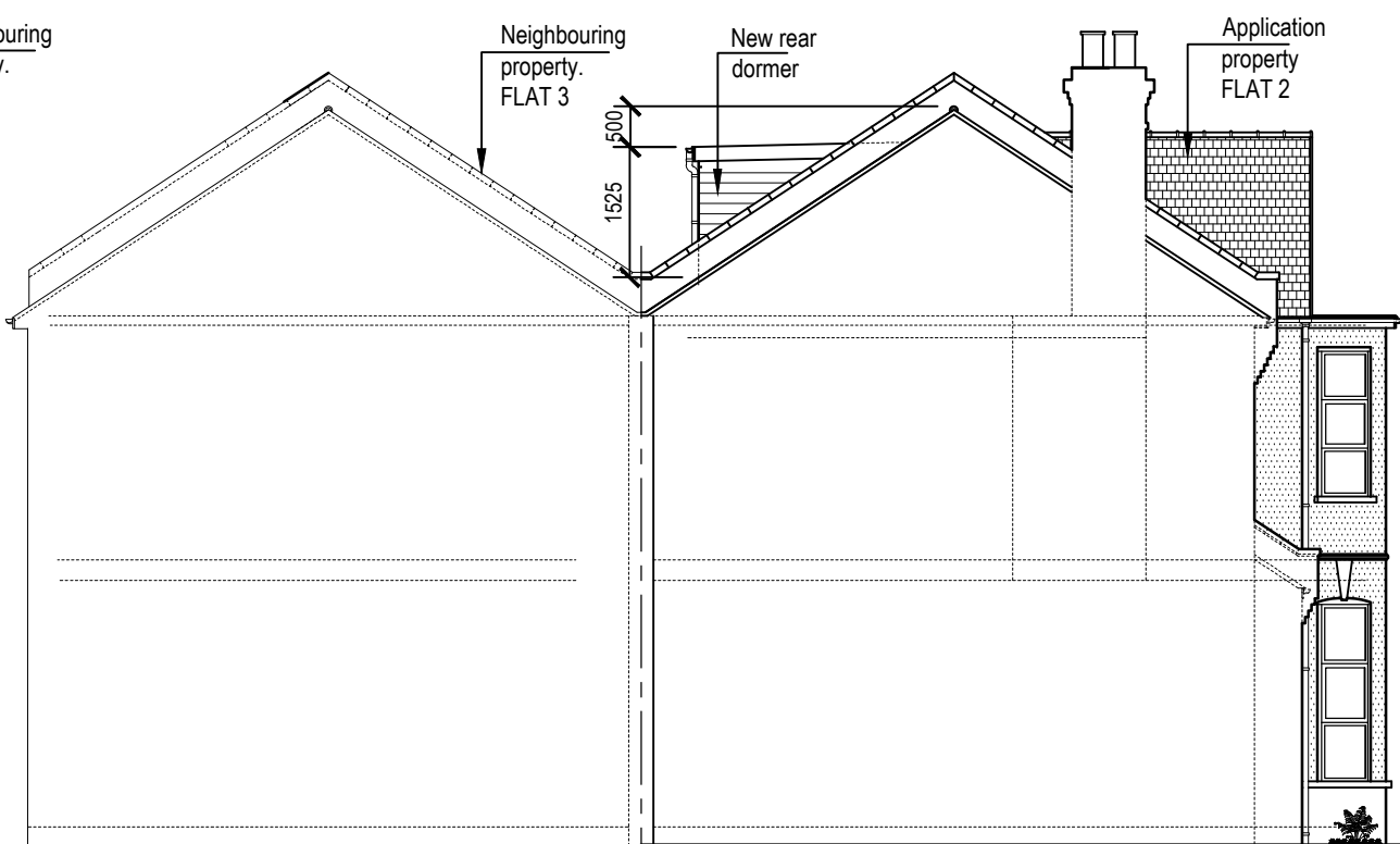
PROPOSED LEFT HAND SIDE (NORTHWEST) ELEVATION
