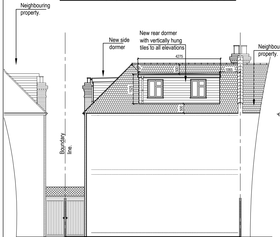
PROPOSED REAR (NORTHEAST) ELEVATION
