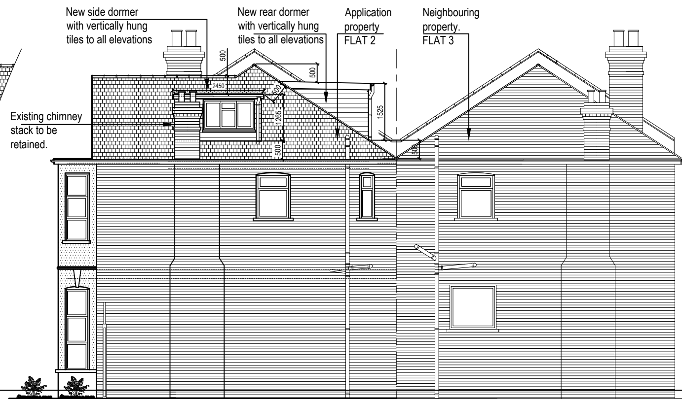
PROPOSED RIGHT HAND SIDE (SOUTHEAST) ELEVATION
