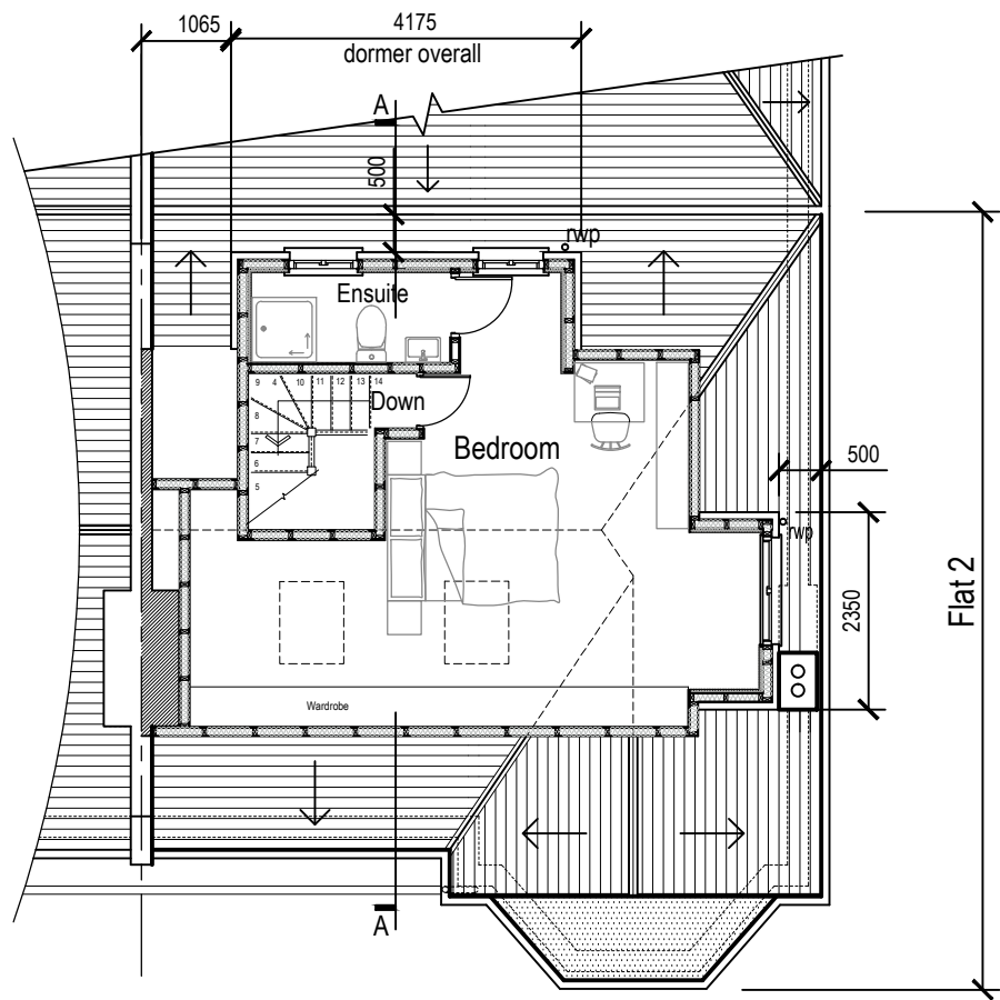
PROPOSED SECOND FLOOR PLAN - FLAT 2
