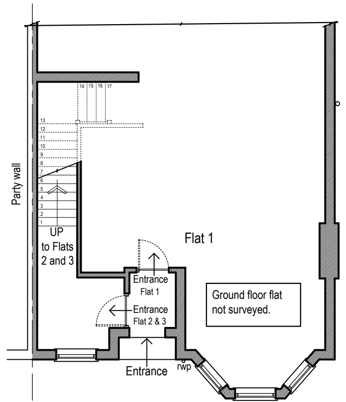
EXISTING GROUND FLOOR PLAN ( PART )
