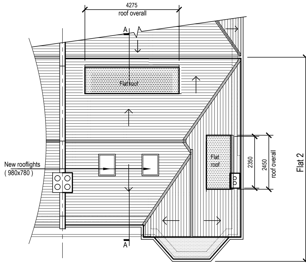
PROPOSED ROOF PLAN - FLAT 2
