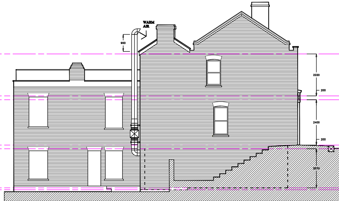
SIDE ELEVATION
