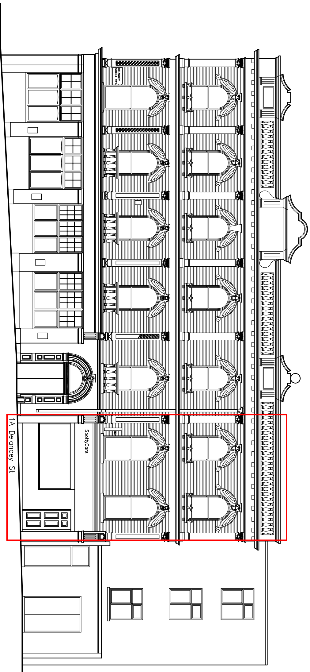
EXISTING FRONT ELEVATION ELEVATION
