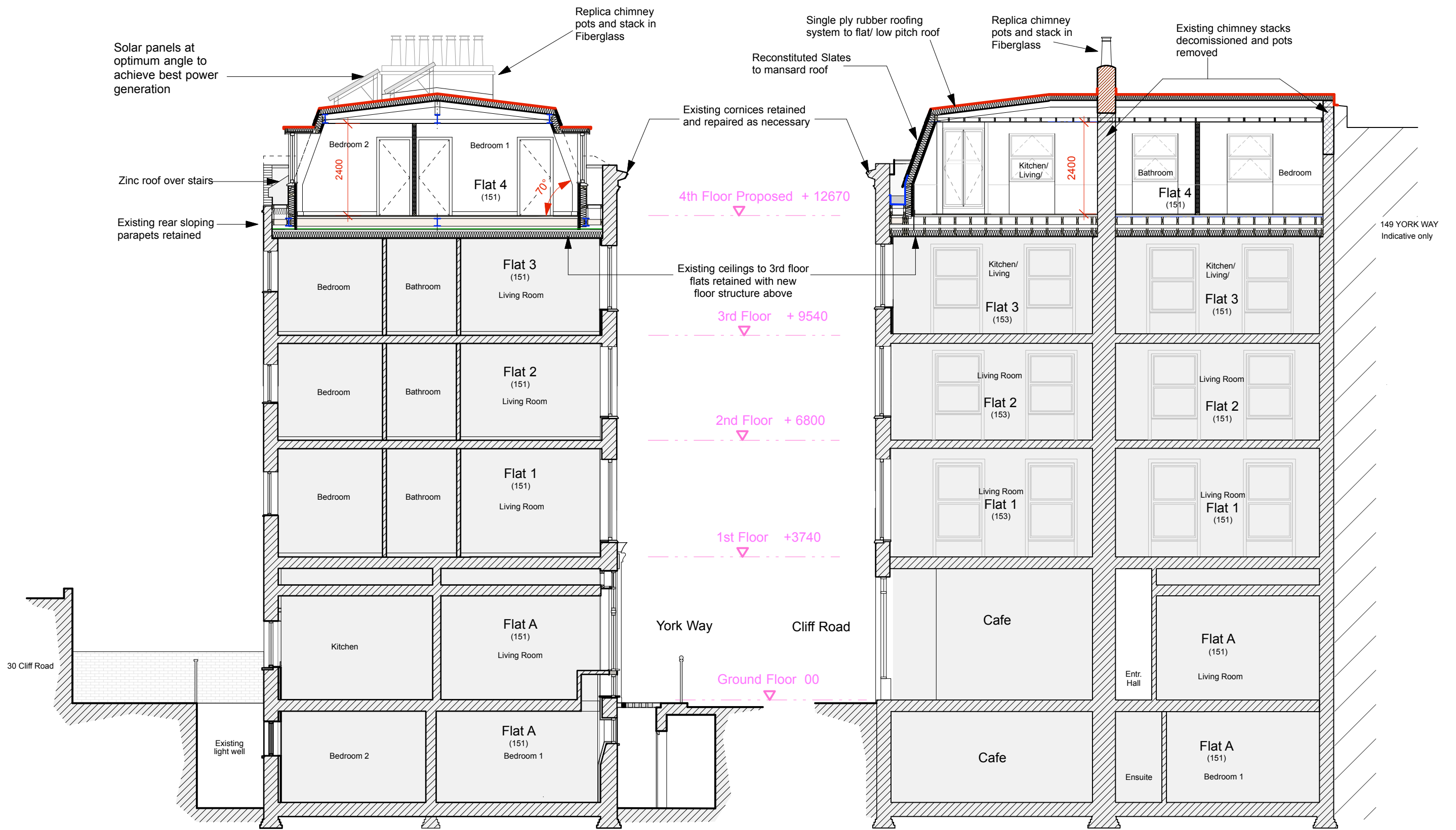
Section A-A - Through 151 York Way
