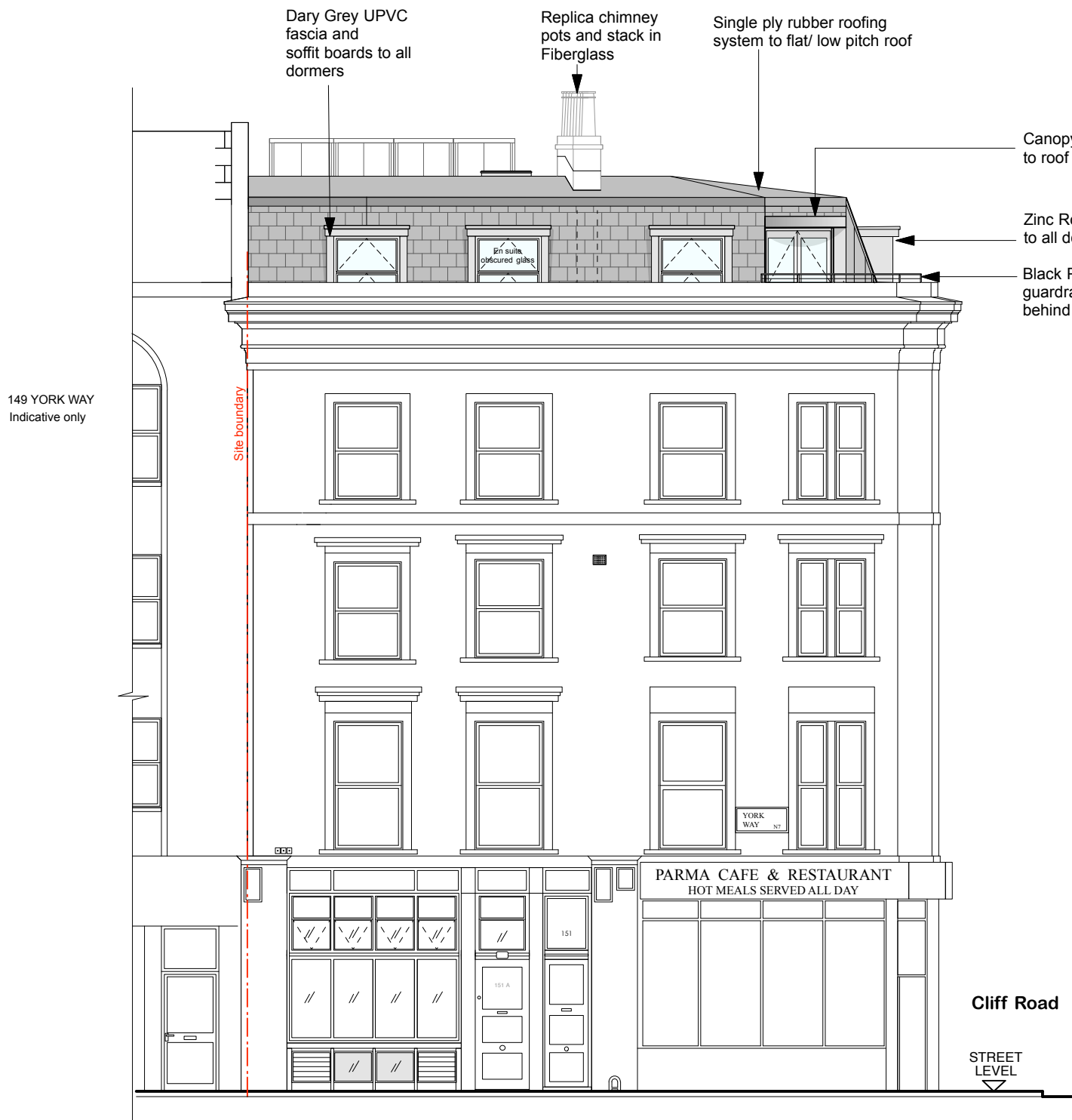
YORK WAY - Front Elevation
