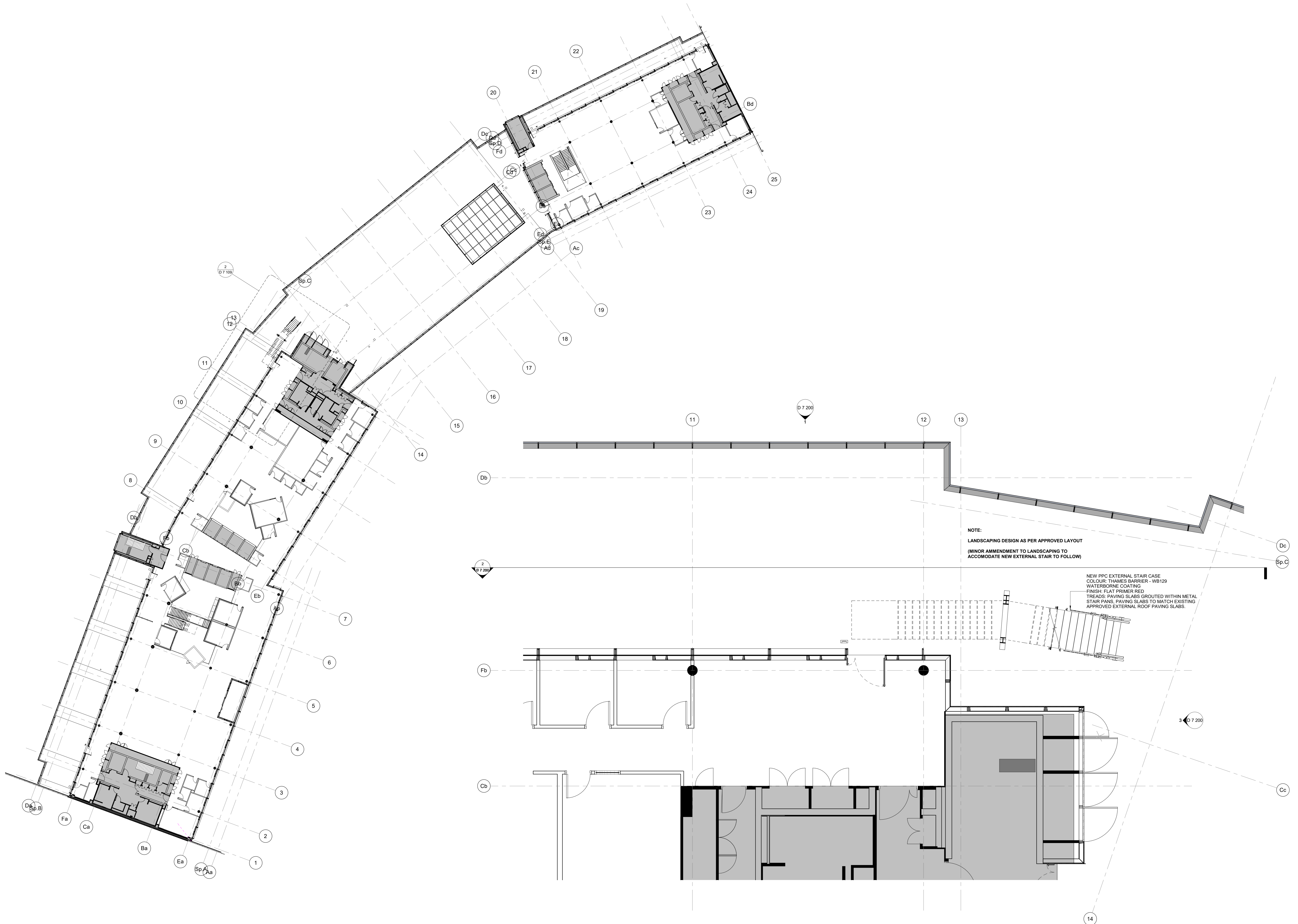
1 Proposed Level 09 Floor Plan 1:250
