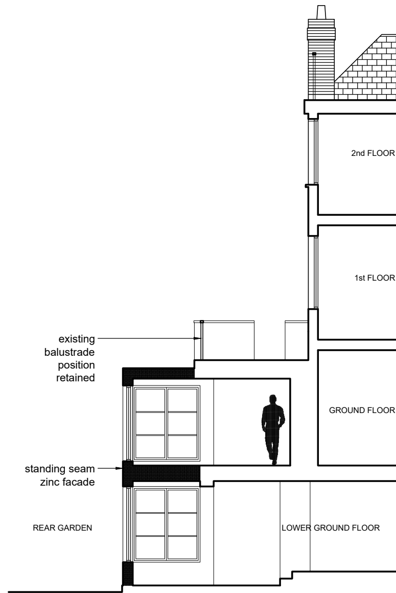
SECTION C
