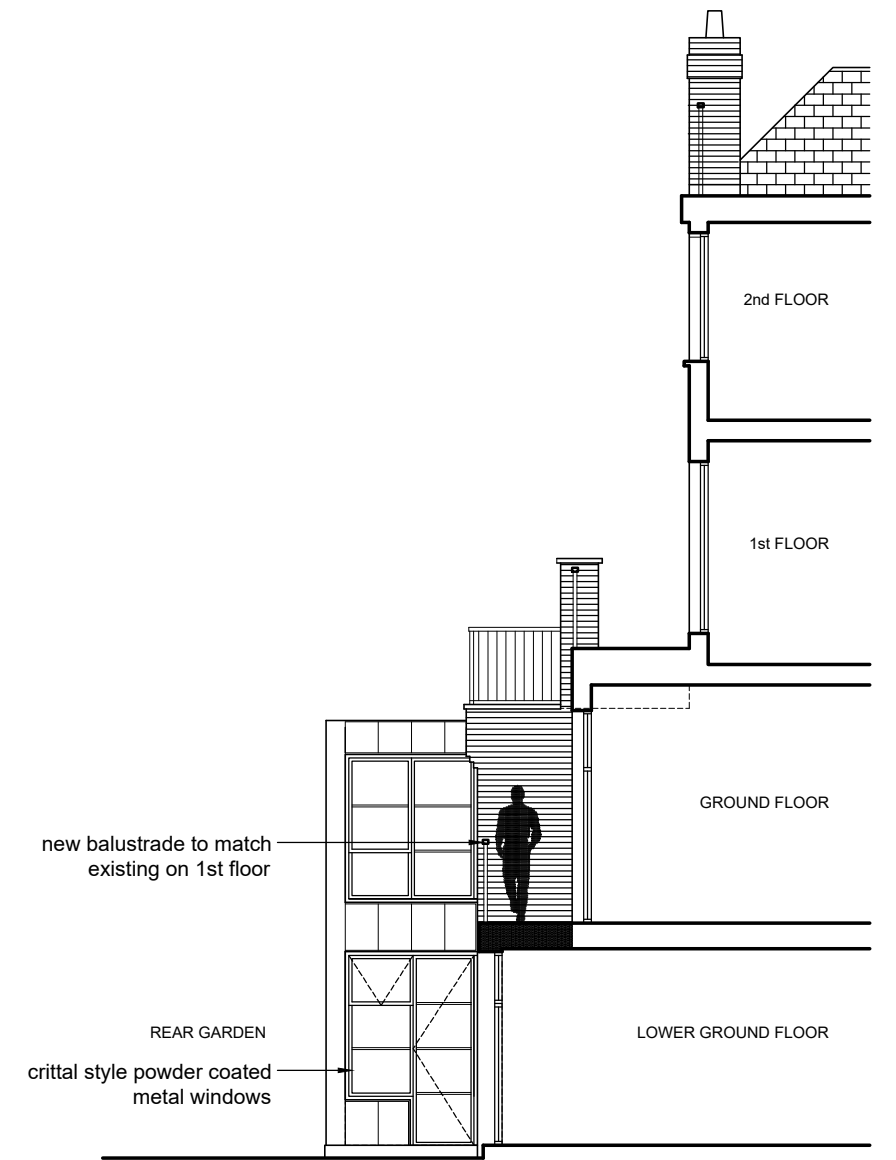
SECTION A
