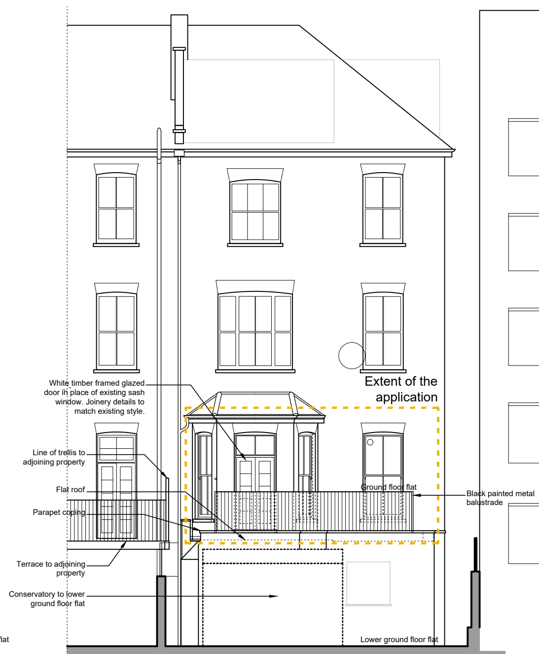
Rear Elevation
