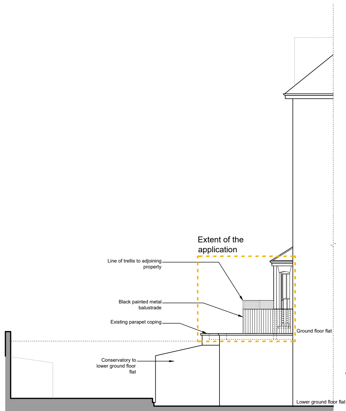
Side Elevation
