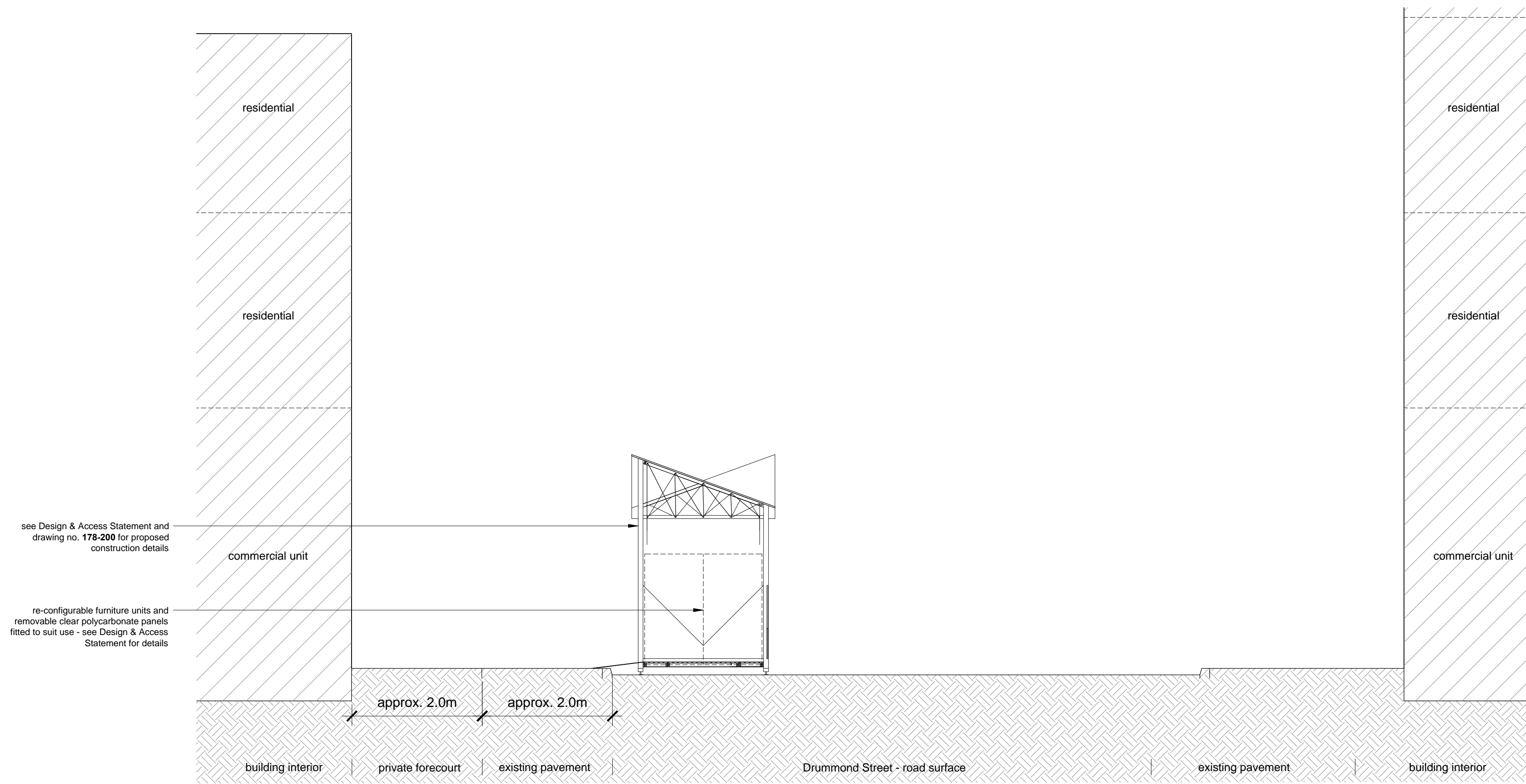
1 Street Section
