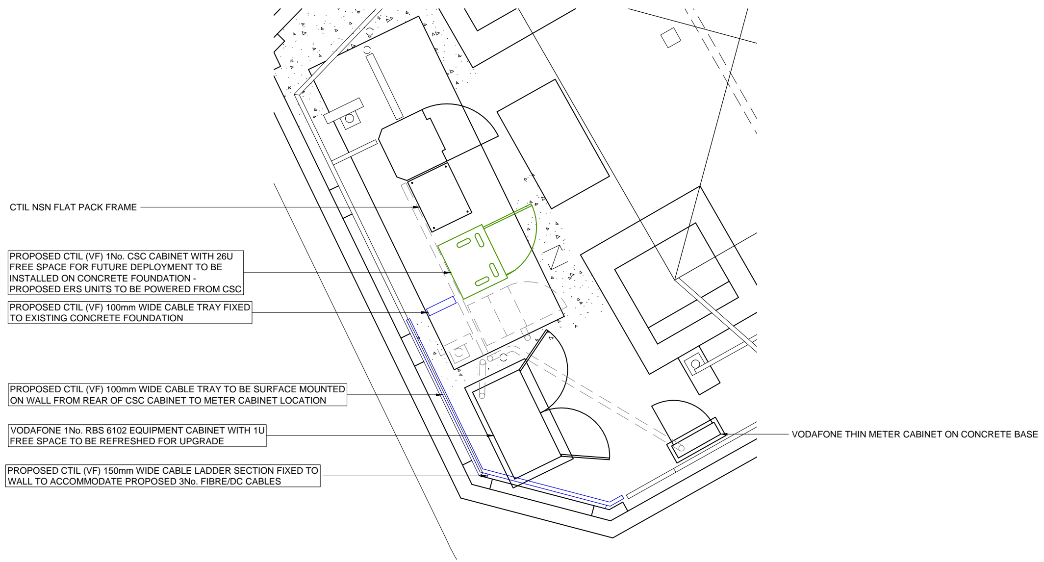
CTIL CABINET LAYOUT
