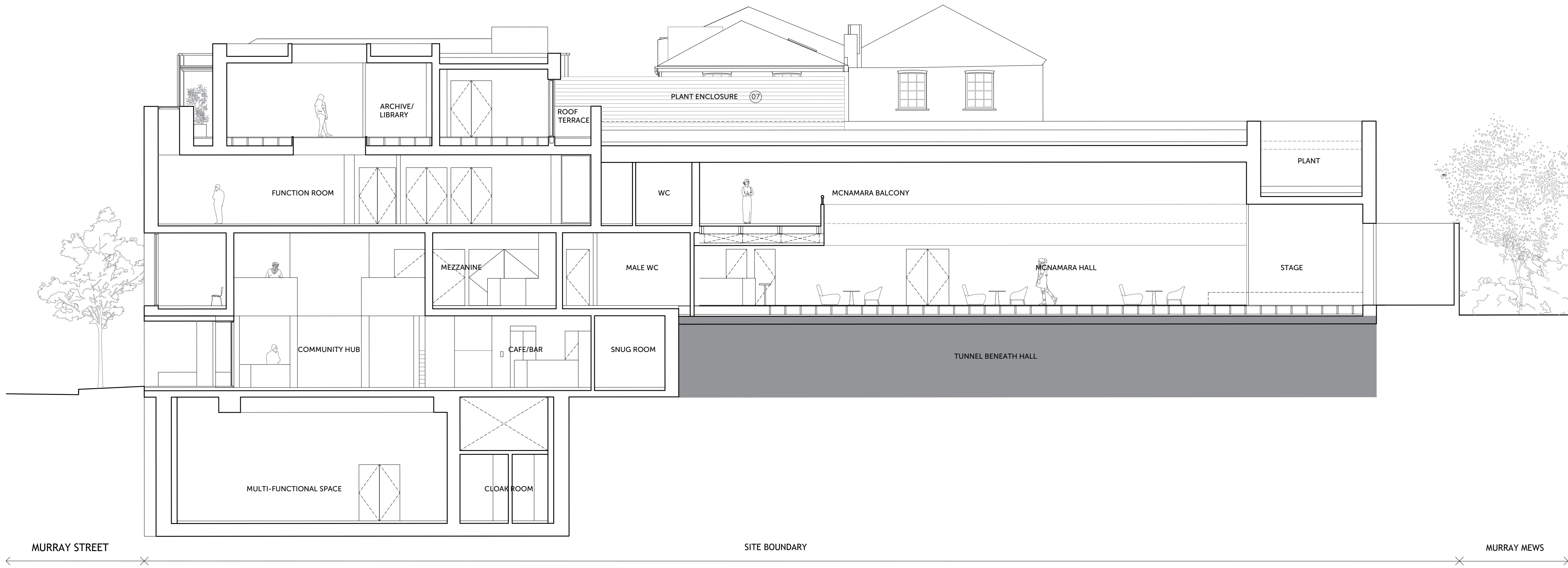
02 PROPOSED SECTION BB
