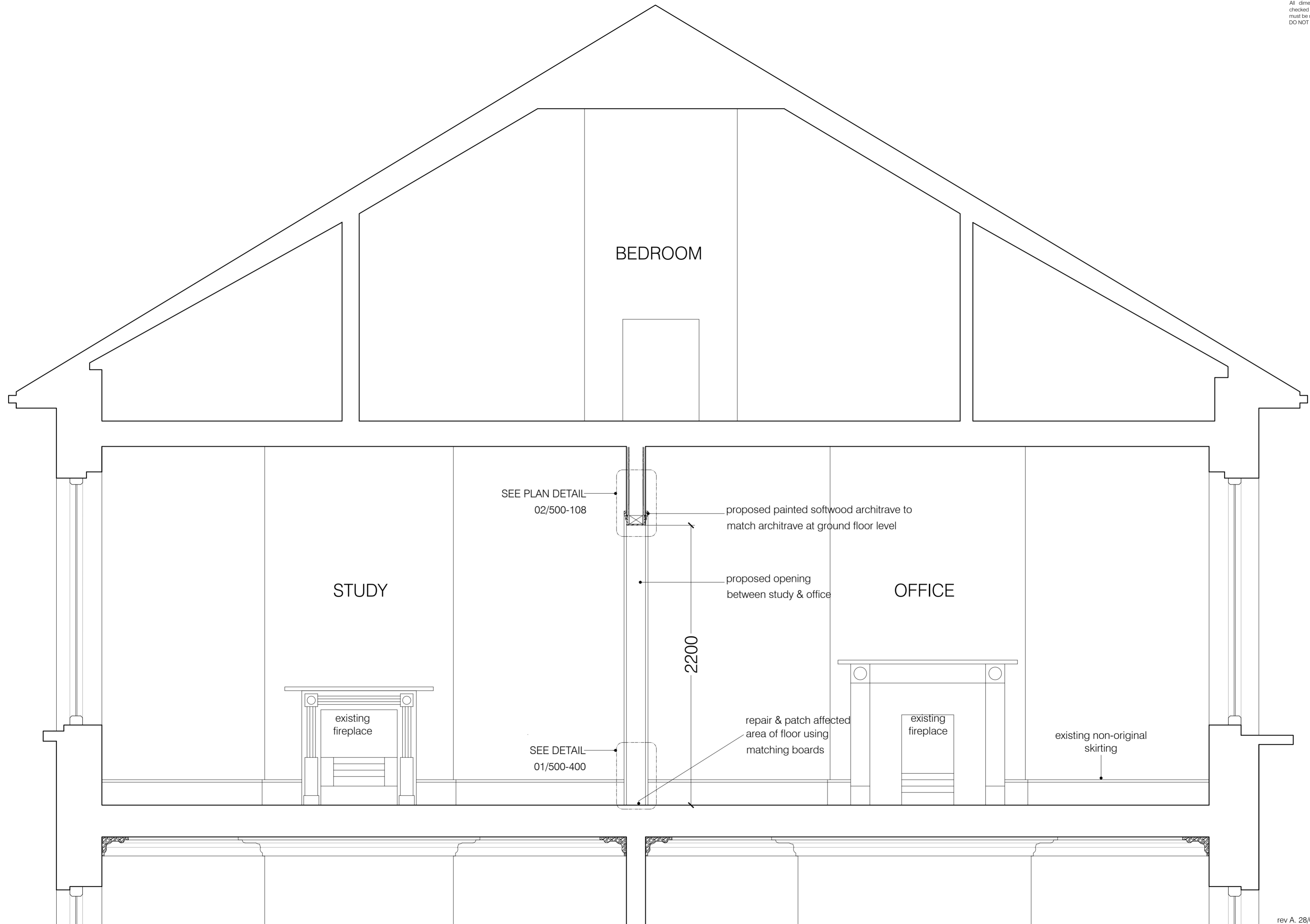
01 PROPOSED SECTION A-A scale 1:20
