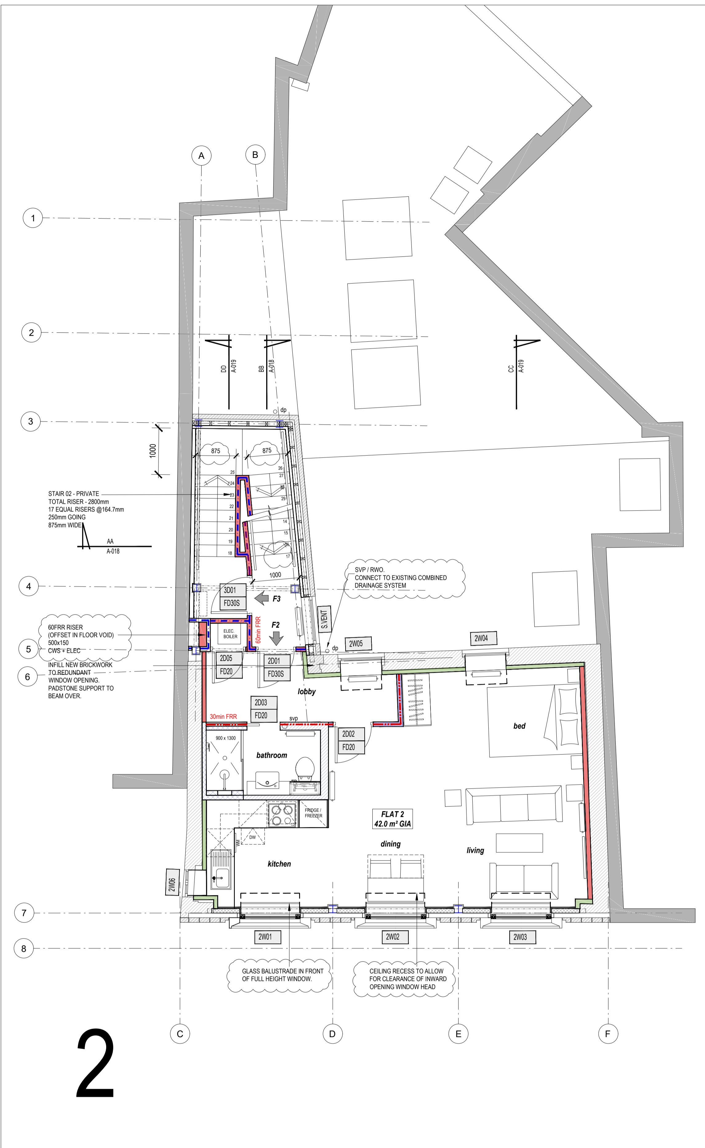
SCALE 1:50@A1 2ND FLOOR - GENERAL ARRANGEMENT
