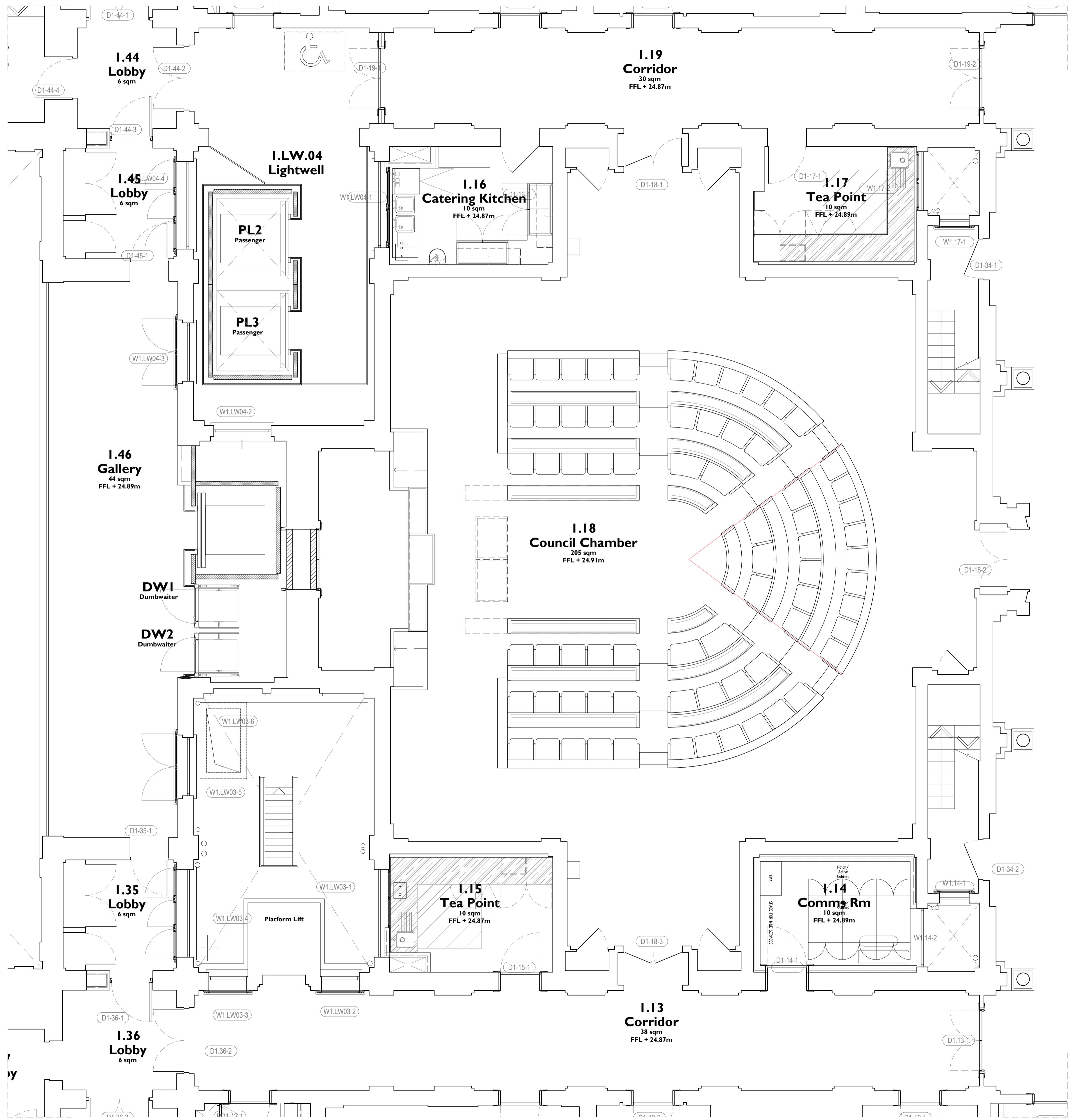
I Council Chamber Proposed Room Plan 4180 1:50 @ A1
