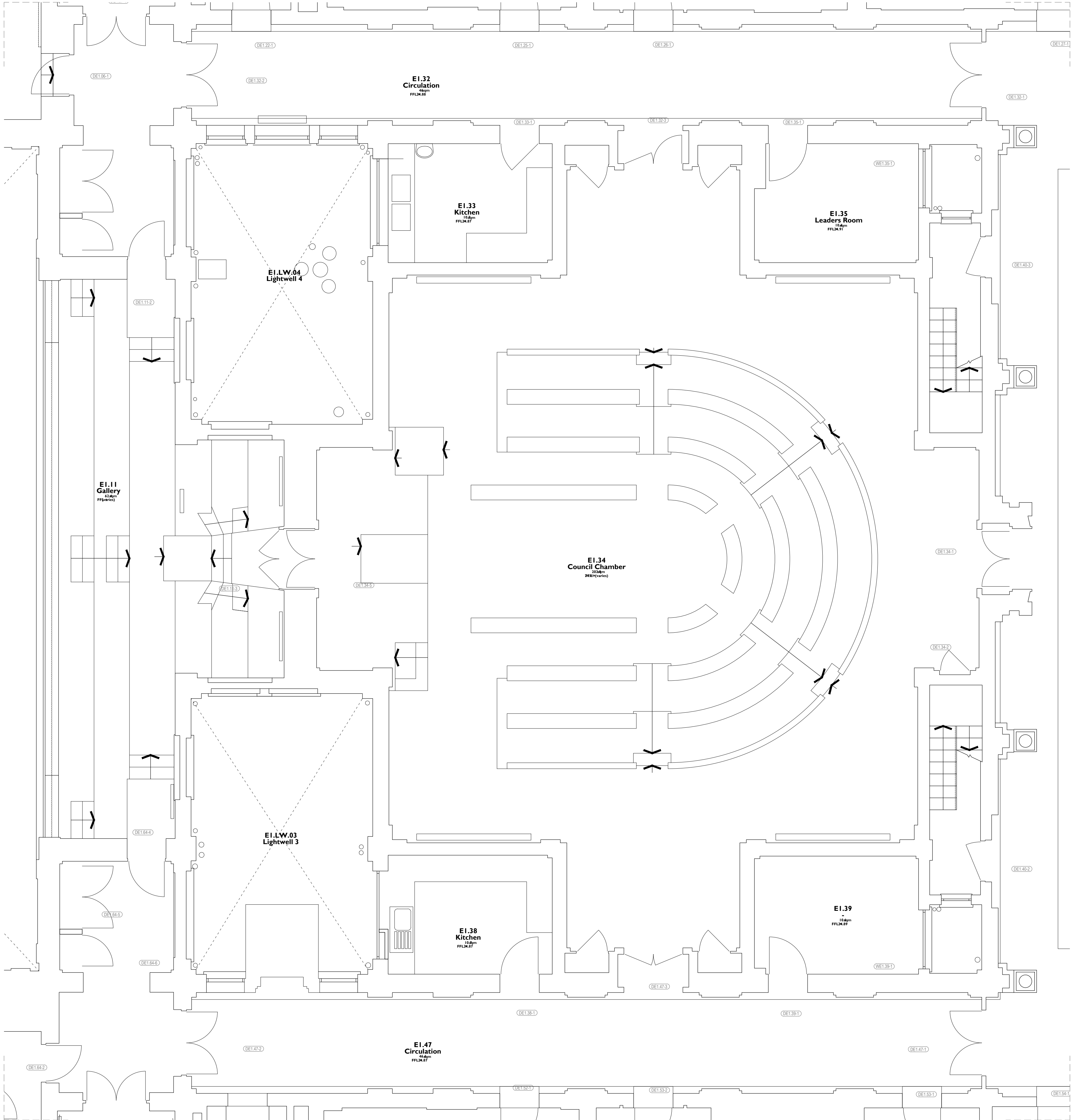
I Council Chamber Existing Room Plan 3341 1:50 @ A1
