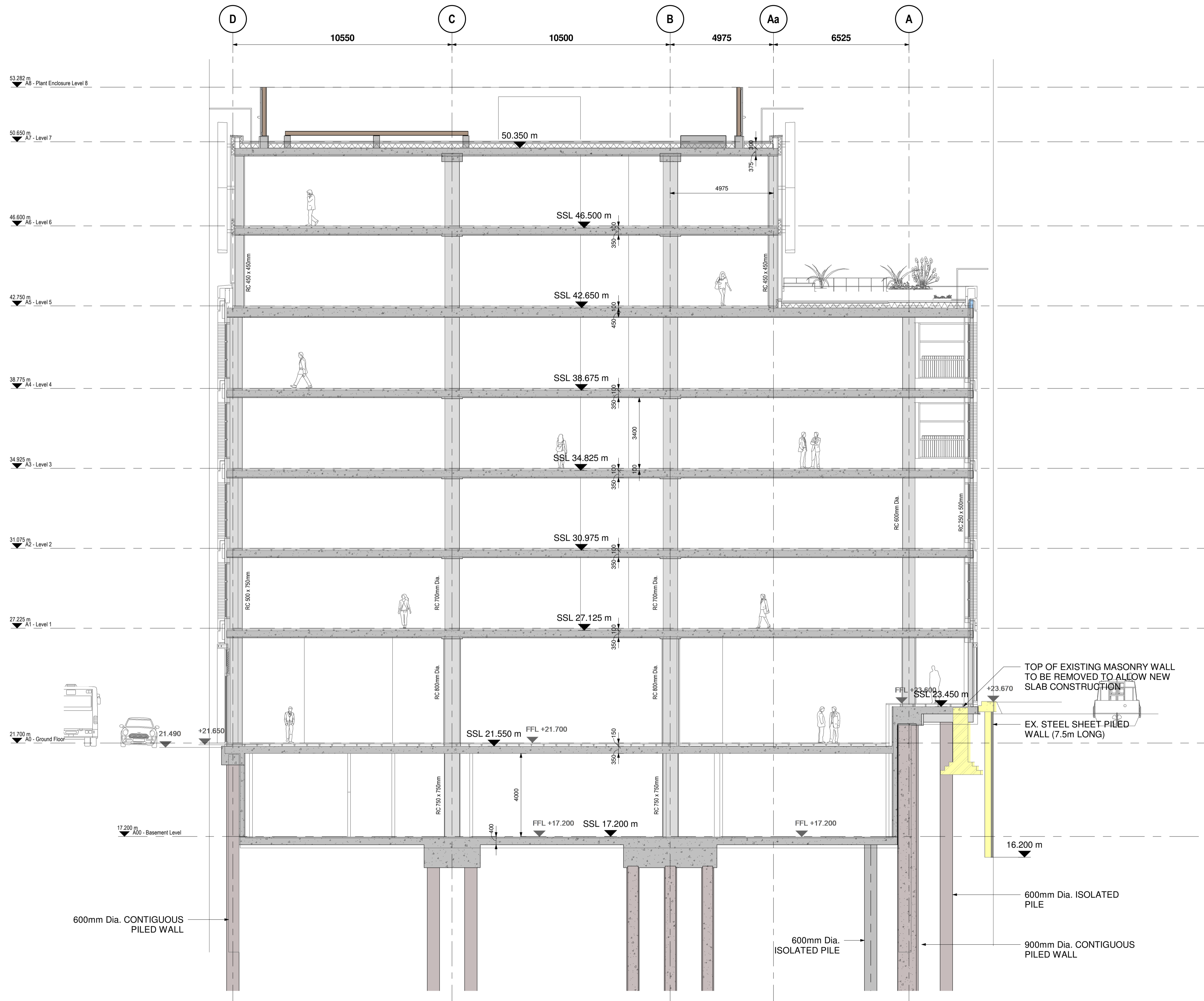
2 PLOT A - Section 2-2 1 : 100
