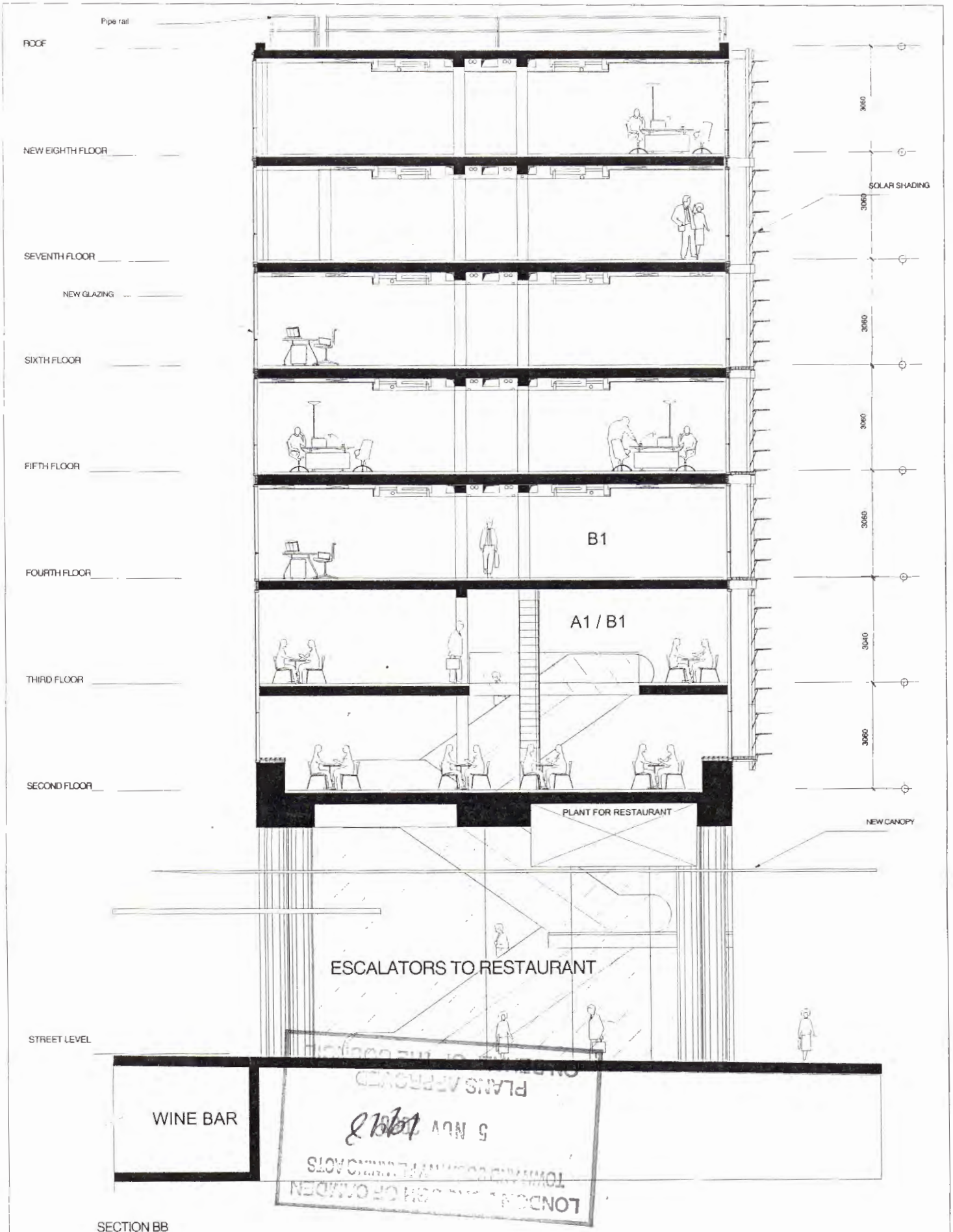
SECTION BB
