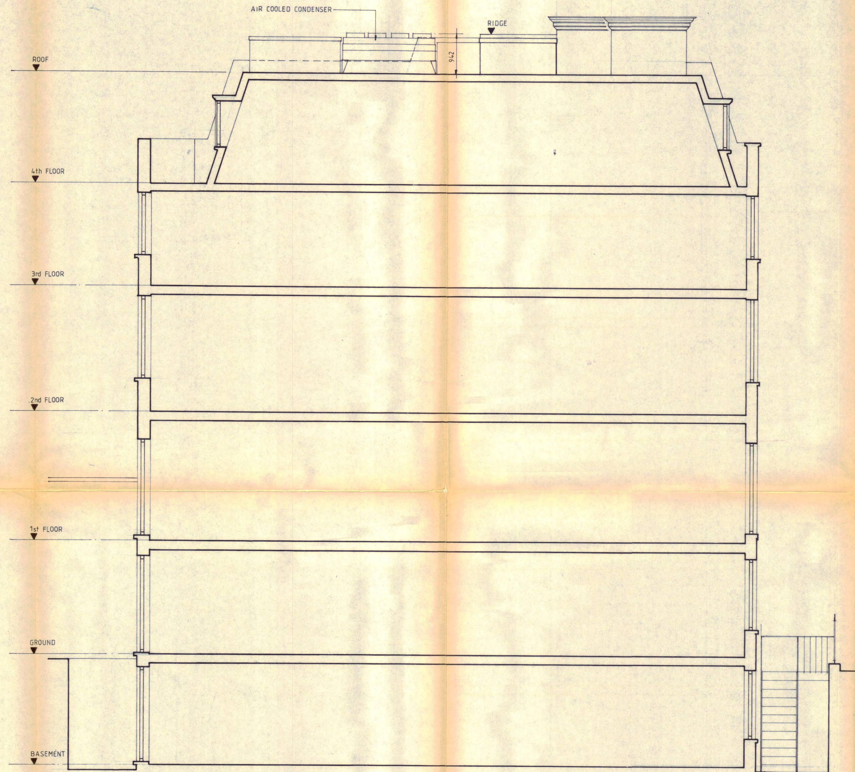
SECTION 1-1
