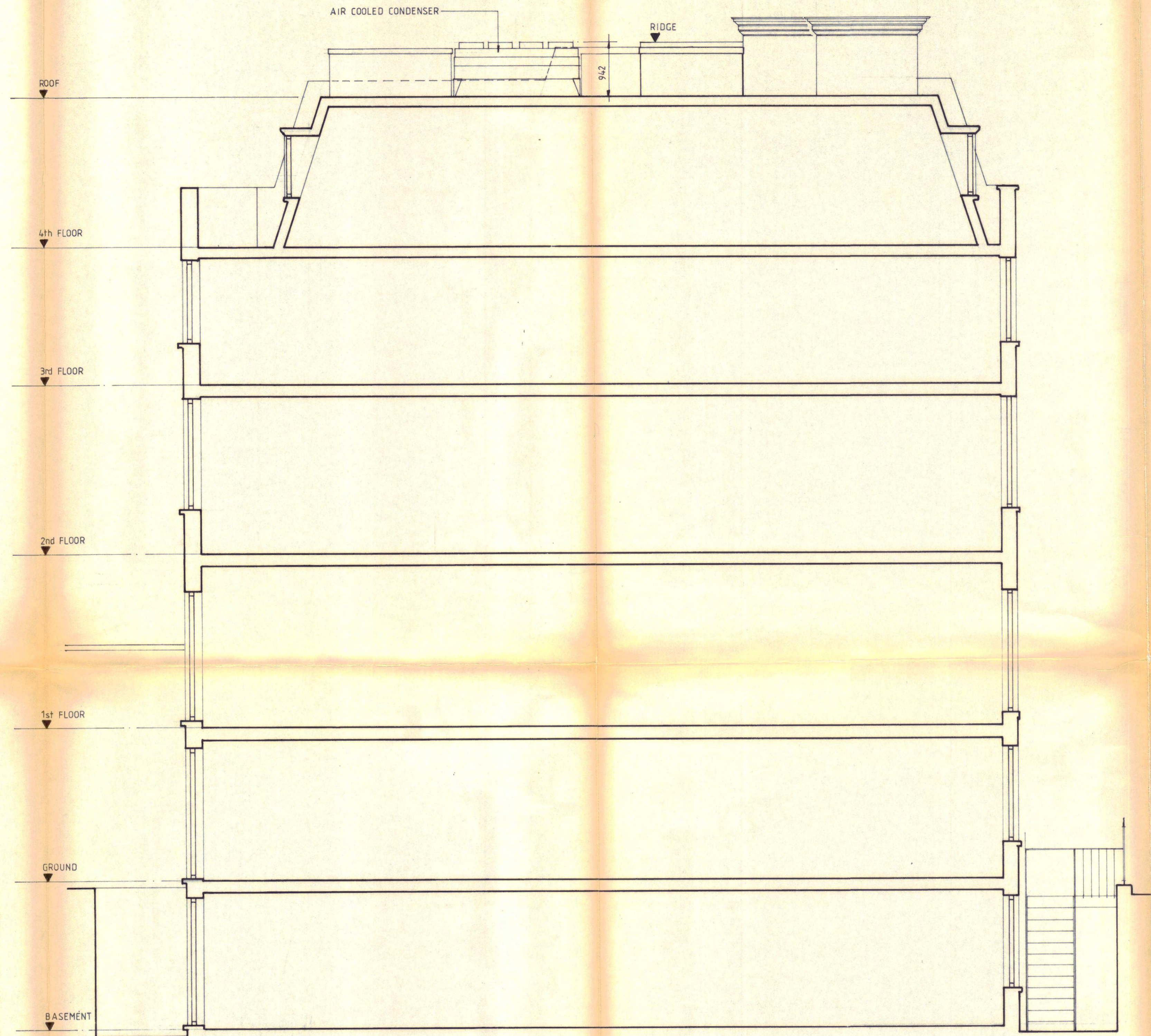
SECTION 1-1
