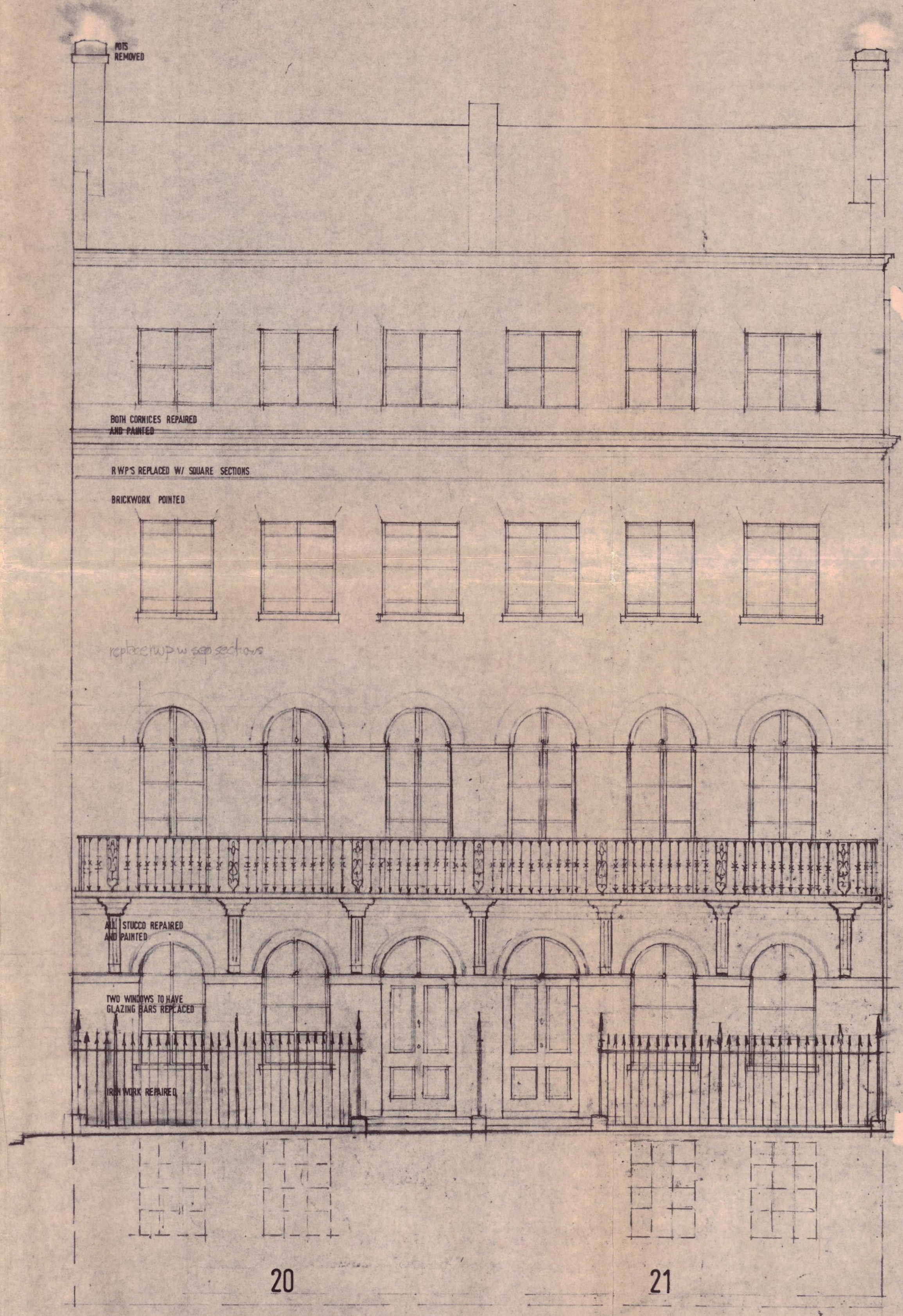
EAST ELEVATION
