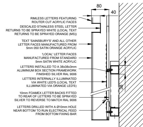
03 PROPOSED FASCIA SIGNAGE DETAIL B-B P128229213 1:10@A3
