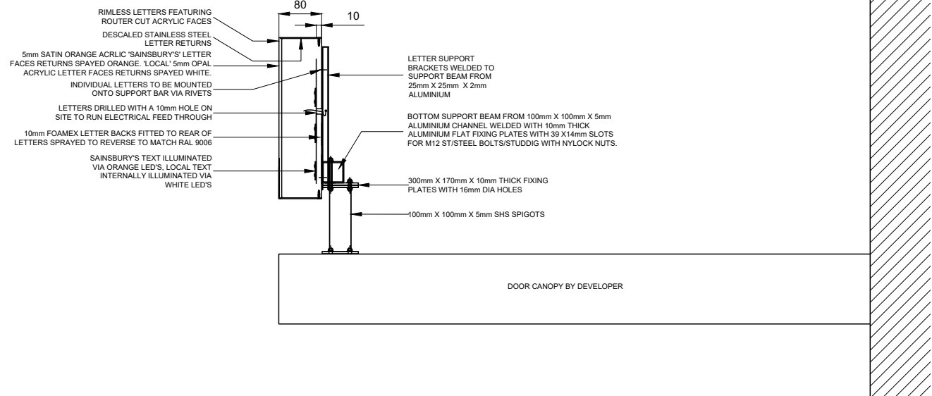
02 PROPOSED FASCIA SIGNAGE DETAIL A-A P128229213 1:10@A3
