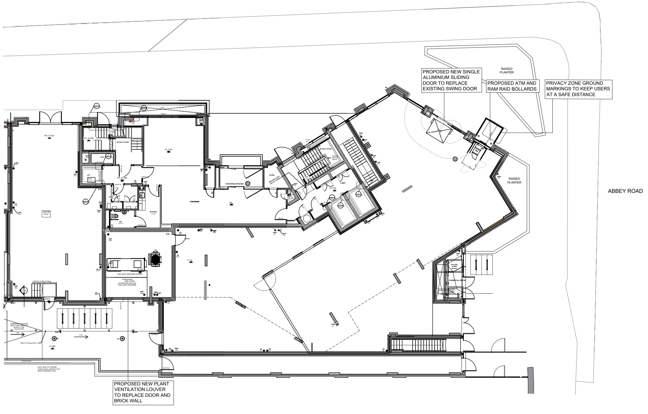
1 PROPOSED GROUND FLOOR PLAN P128229110 1:200@A3
