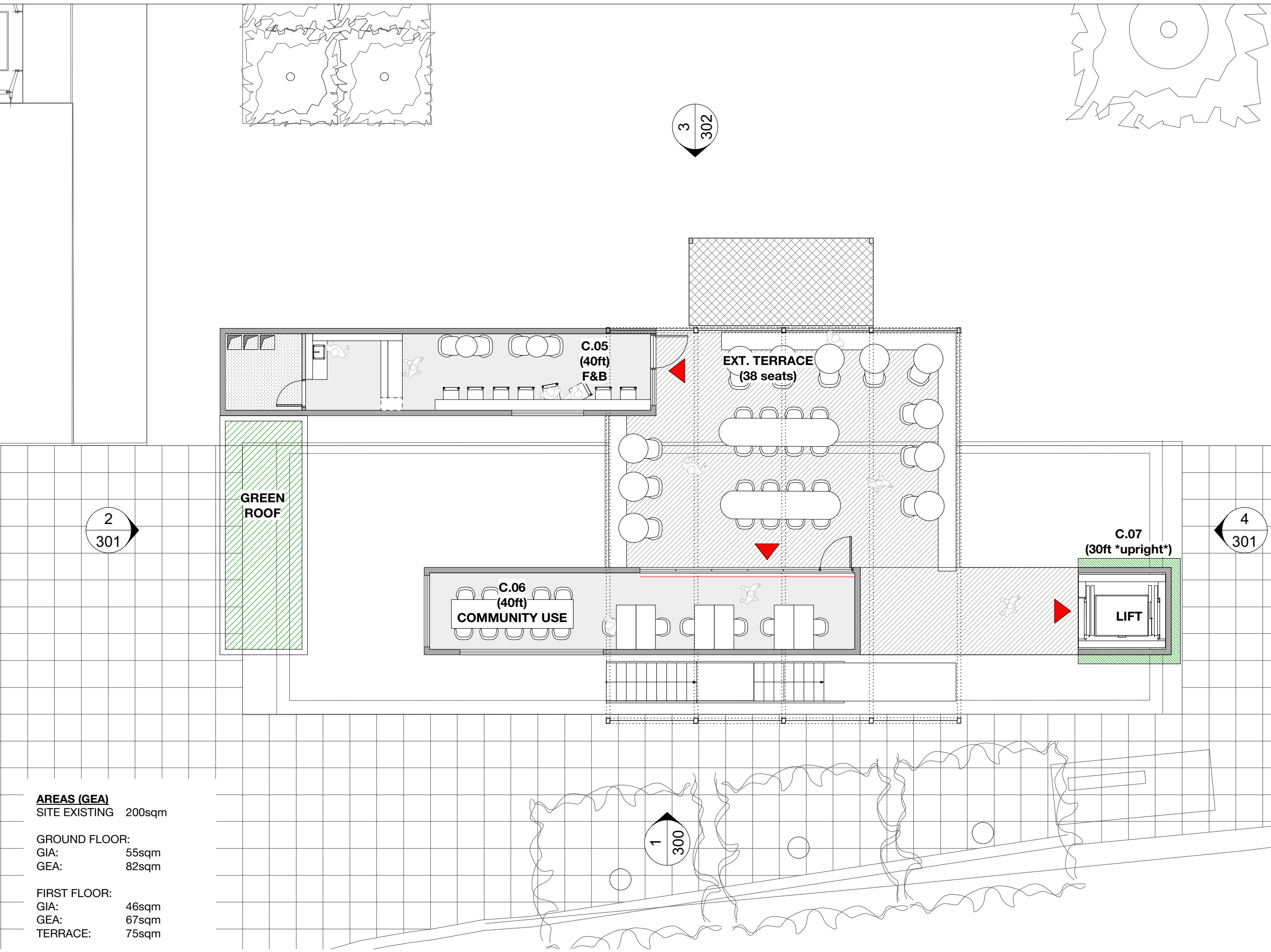
1 PROPOSED FIRST FLOOR PLAN 1:100 @ A3
