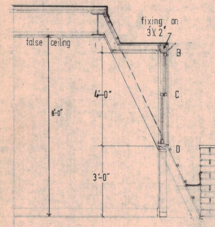
SECTION
