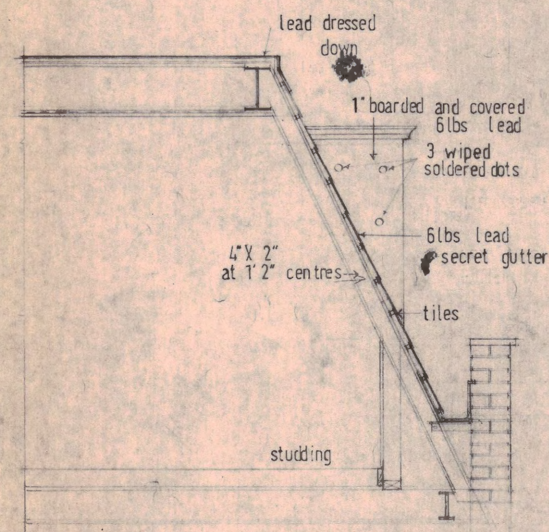
SIDE ELEVATION
