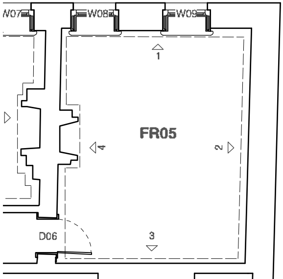
PLAN FR05 @ 1:100
