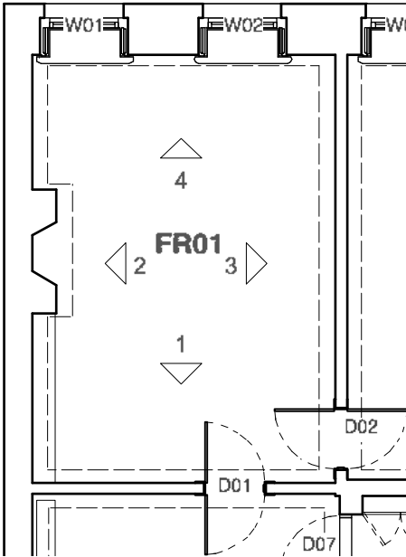
PART PLAN @ 1:100
