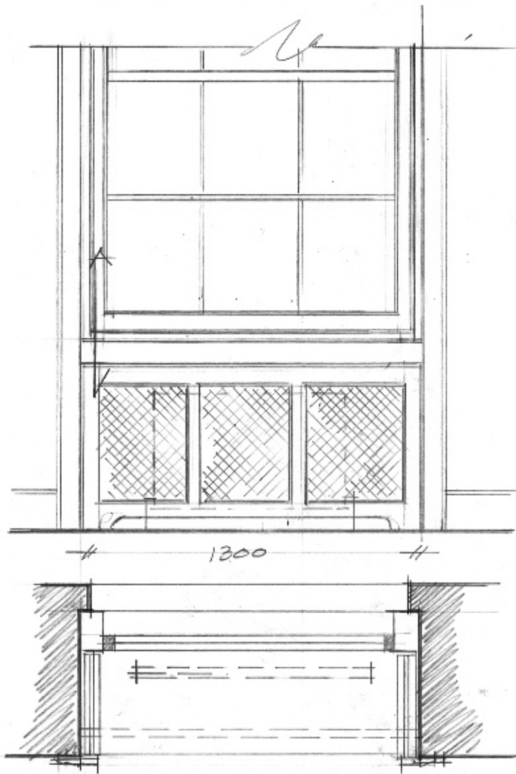
PLAN & ELEVATION
