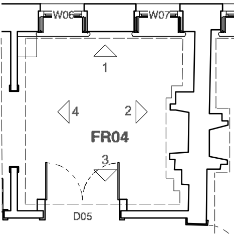
PART PLAN @ 1:100
