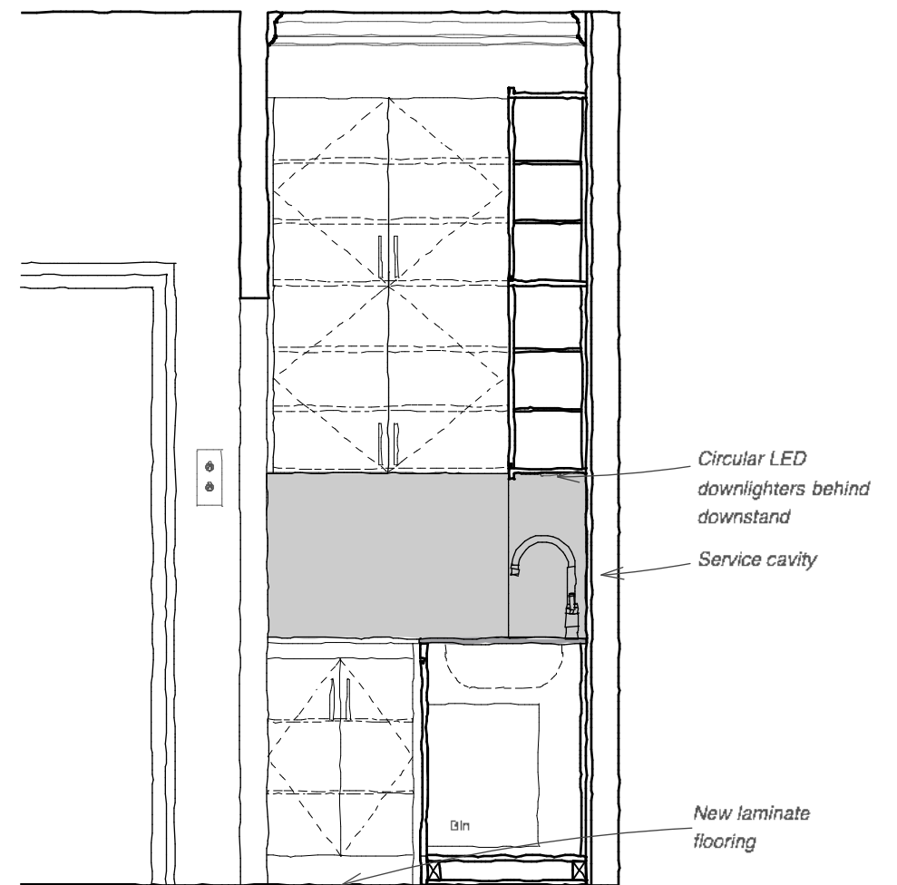
SECTION C-C
