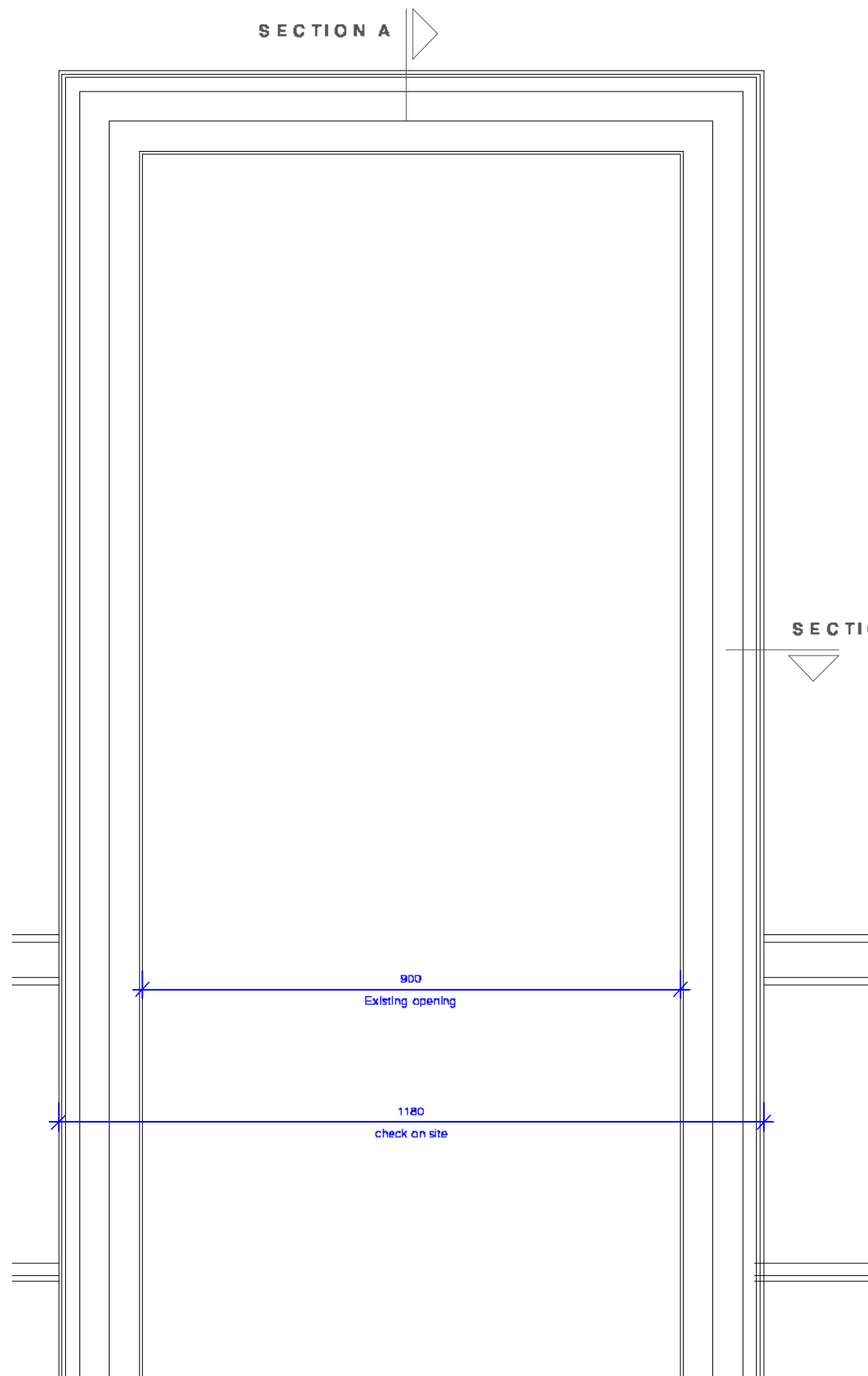
ELEVATION 1:10
