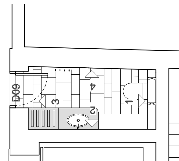
PLAN FR10 @ 1:50
