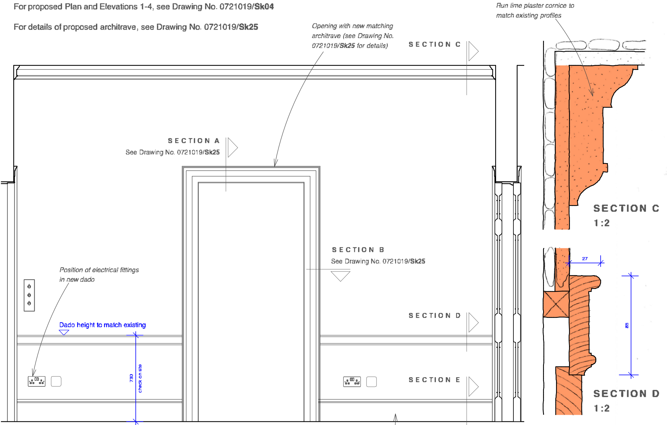
PROPOSED ELEVATION 1 1:20
