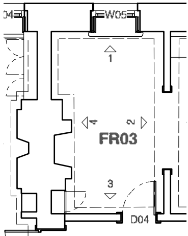
PART PLAN @ 1:100
