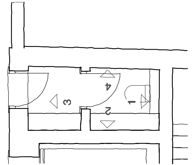
PLAN FR10 @ 1:50
