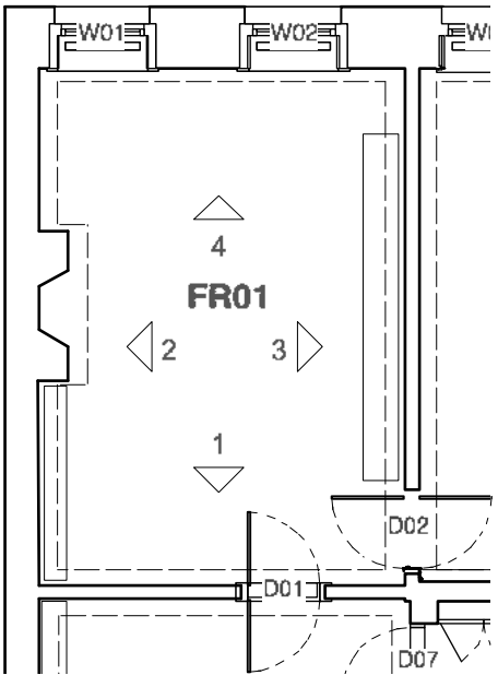
PART PLAN @ 1:100
