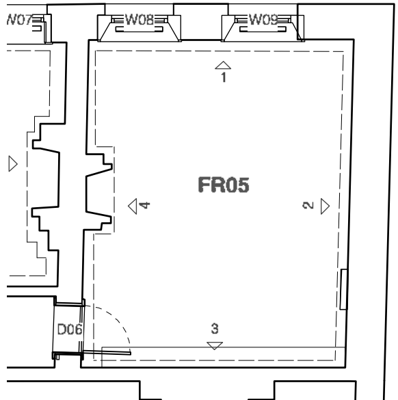
PLAN @ 1:100
