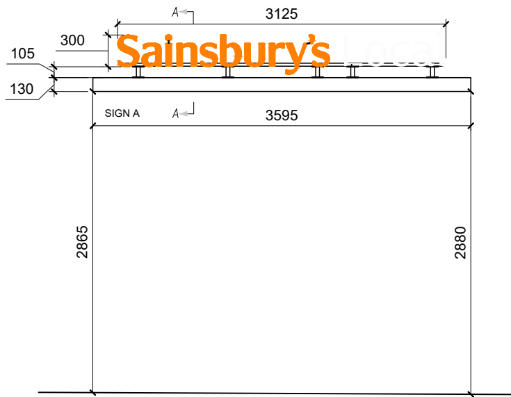
01 PROPOSED FASCIA SIGNAGE-INTERNALLY ILLUMINATED- ILLUMINATION LEVEL - 375 cd/m 2 P128229213 1:50@A3
