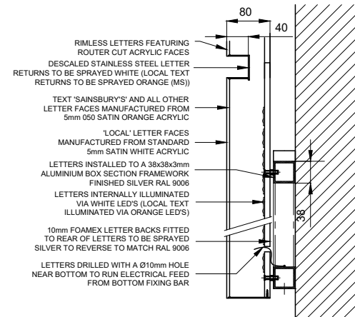
02 PROPOSED FASCIA SIGNAGE DETAIL A-A P128229213 1:10@A3
