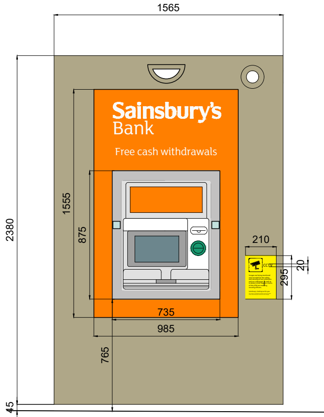
06 PROPOSED ATM SURROUND P128229213 1:25@A3
