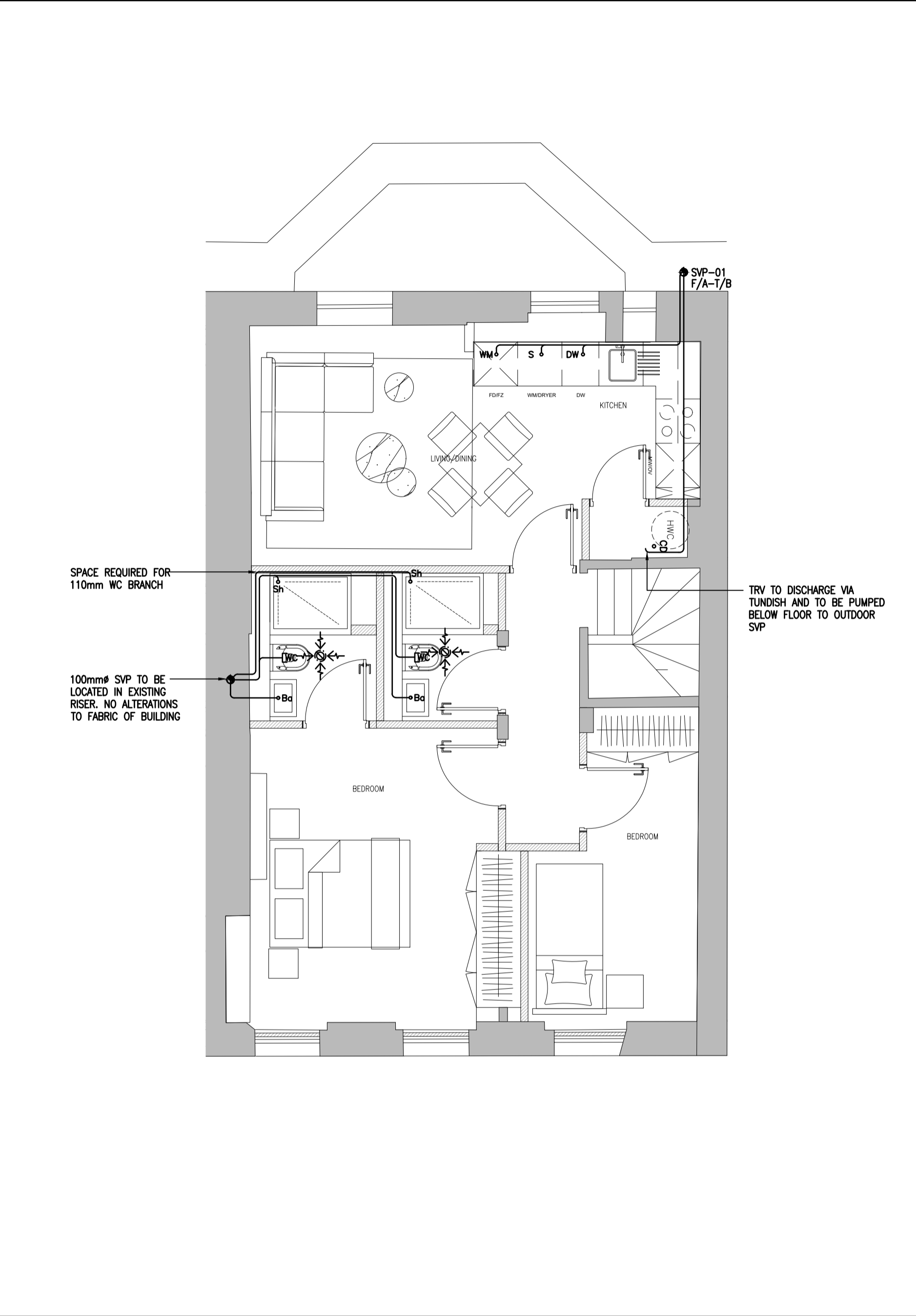
SOIL & WASTE LAYOUT
