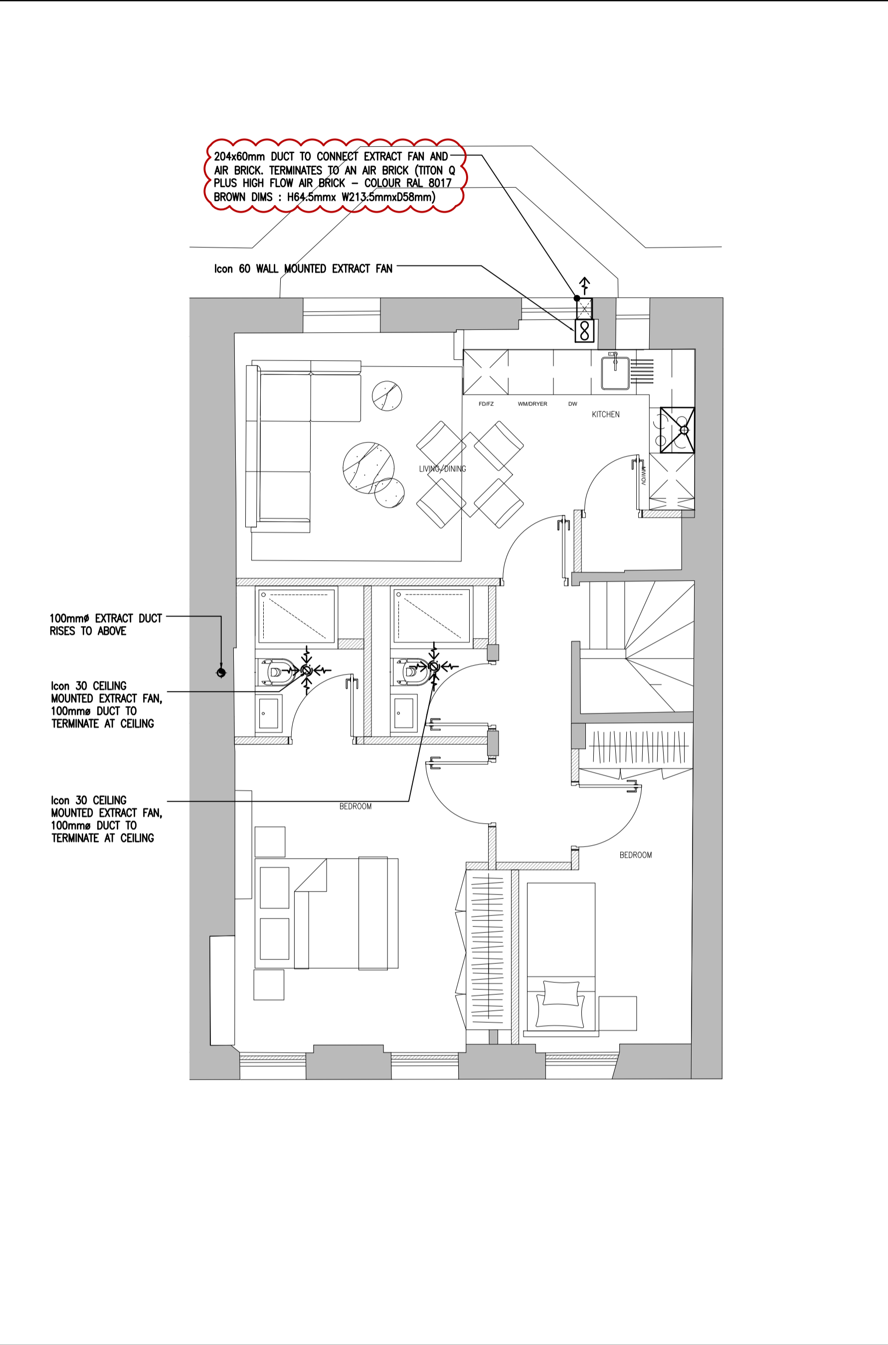
VENTILATION LAYOUT
