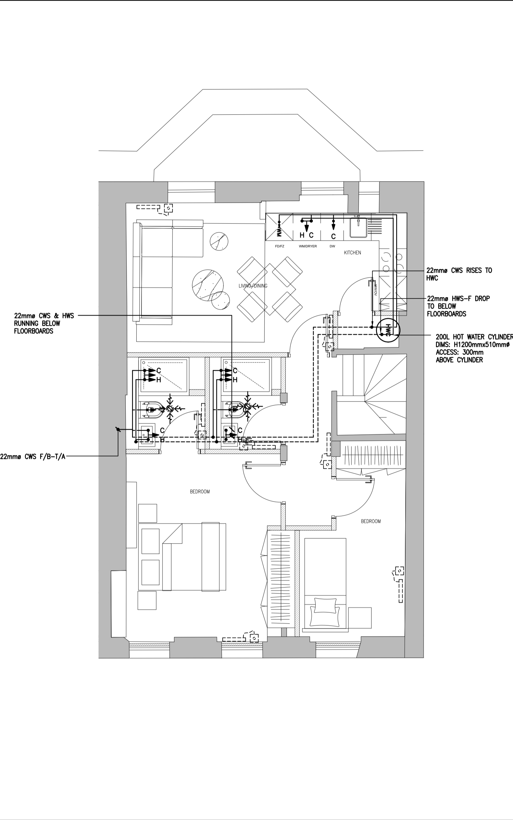
WATER & HEATING LAYOUT
