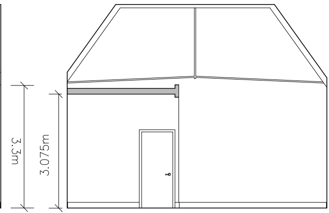
PROPOSED SECTION C – C
