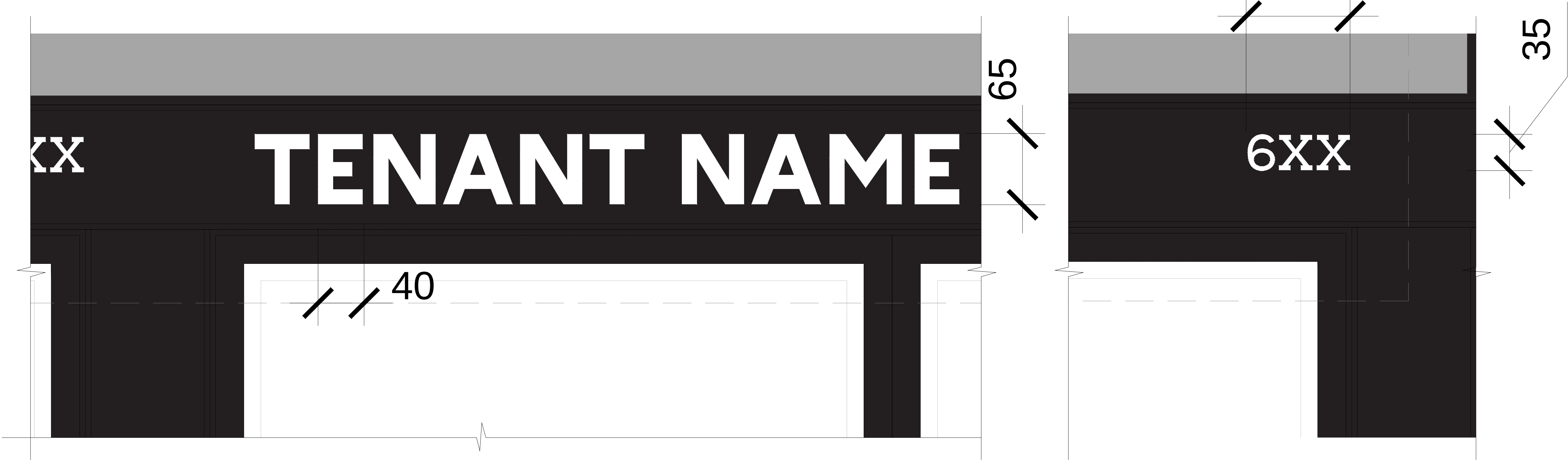
02 SIGNAGE- DETAIL 2 07-130 1:2
