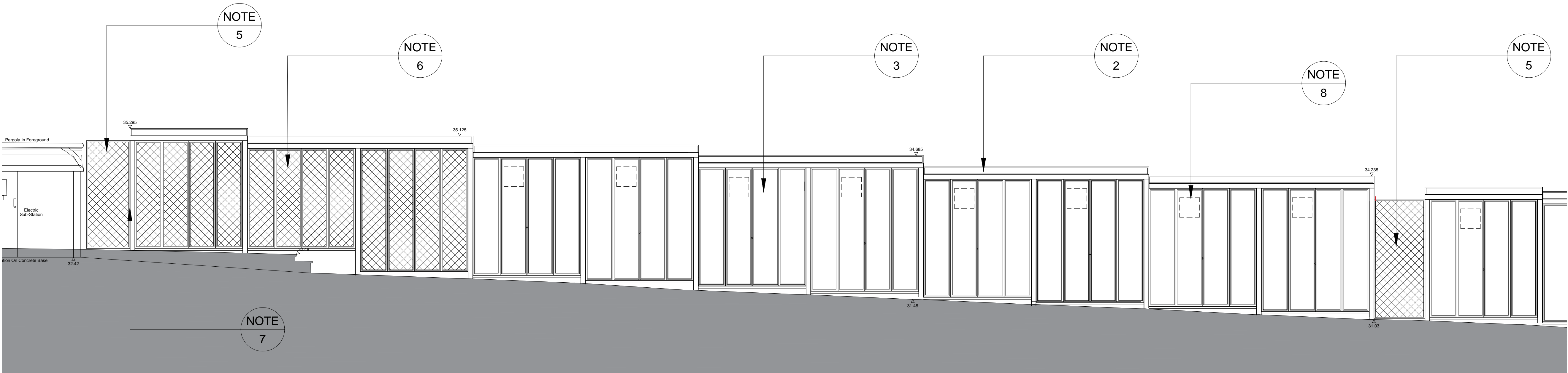
01 PROPOSED TYPICAL SOUTH ELEVATION
