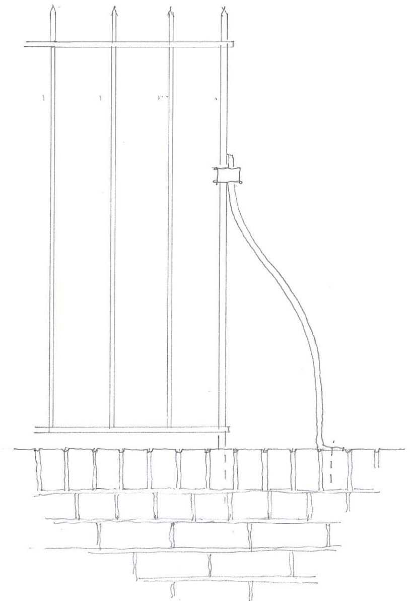
TERMINATION DETAIL
