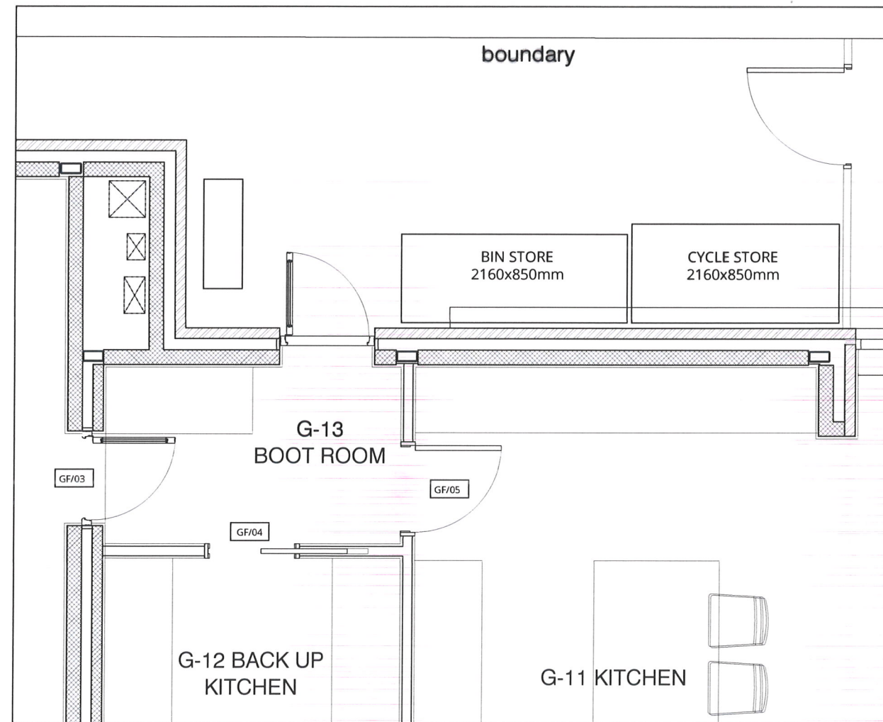
Partial Ground Floor Plan SCALE 1:50
