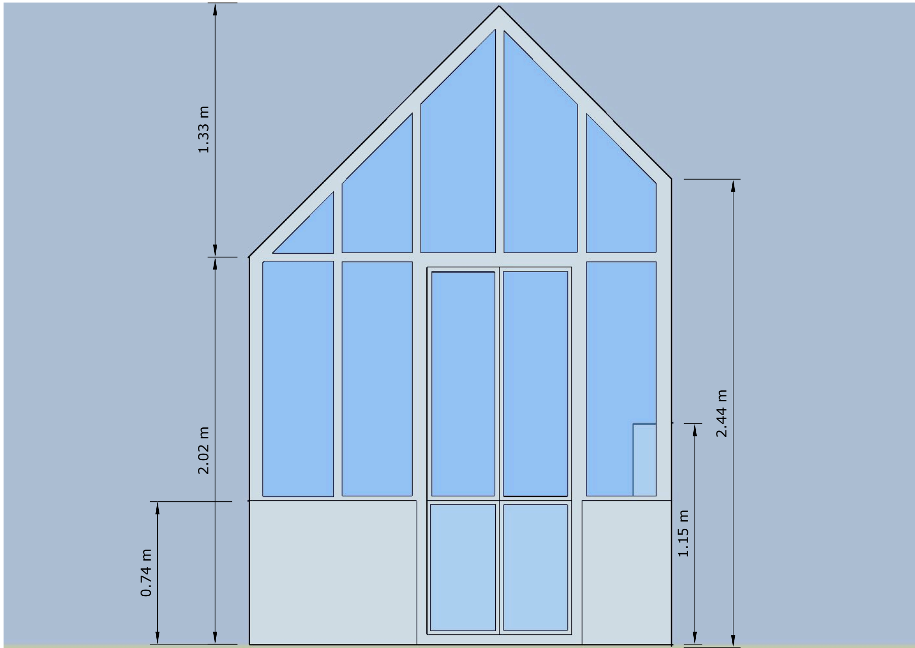
3 Tanza Rd Glasshouse -W Elevation SCALE 1:20
