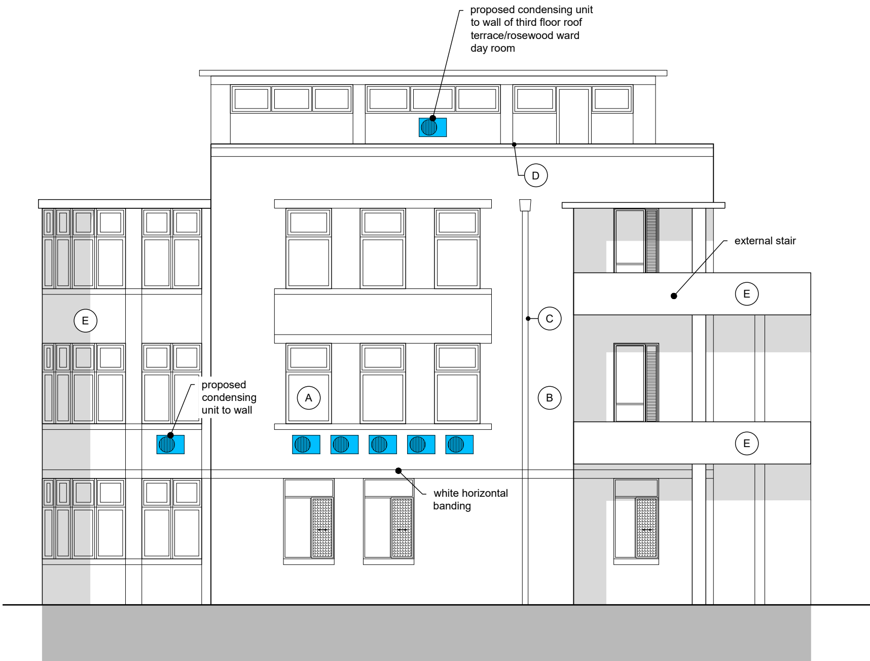
3 Proposed - South Elevation
