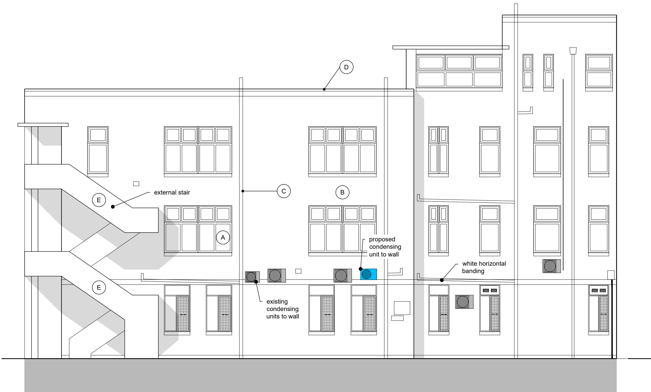
2 Proposed - North-East Elevation
