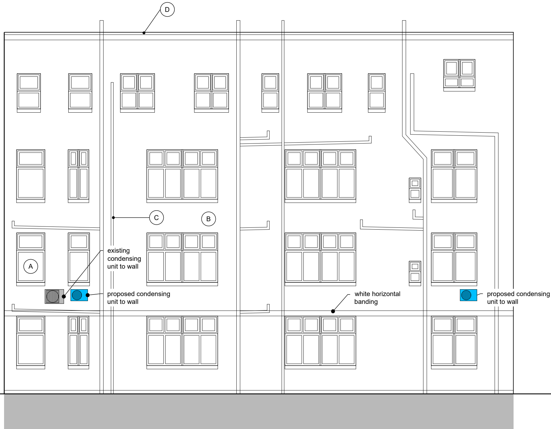
1 Proposed - South-East Elevation
