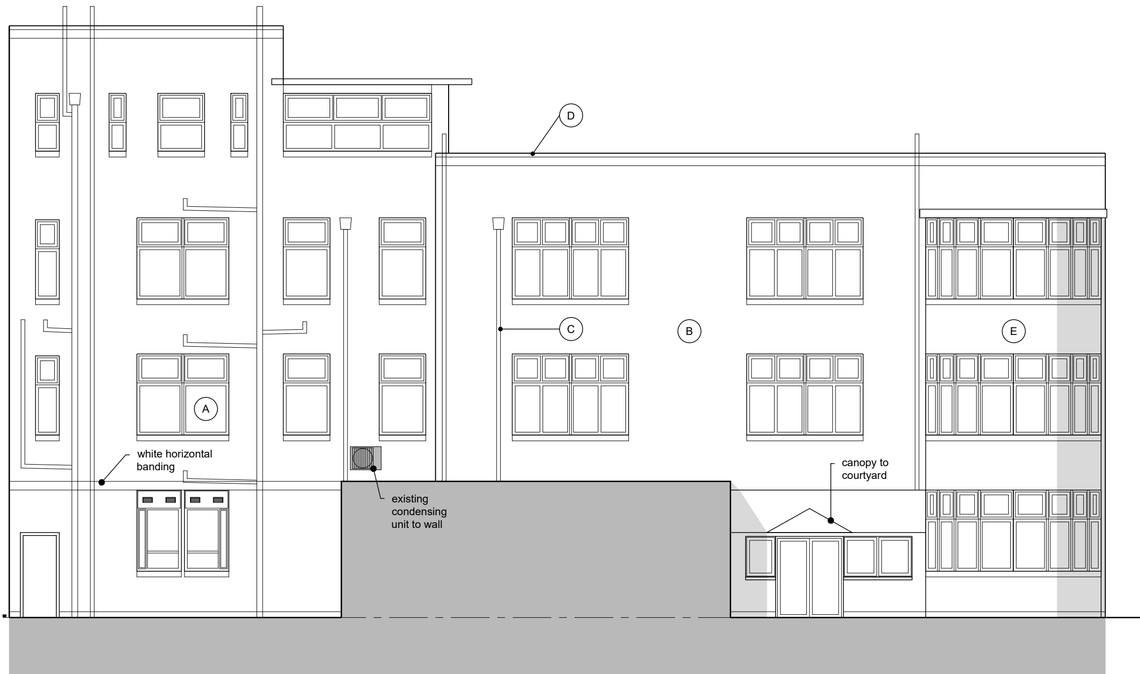
4 Existing - South-West Elevation 1:100
