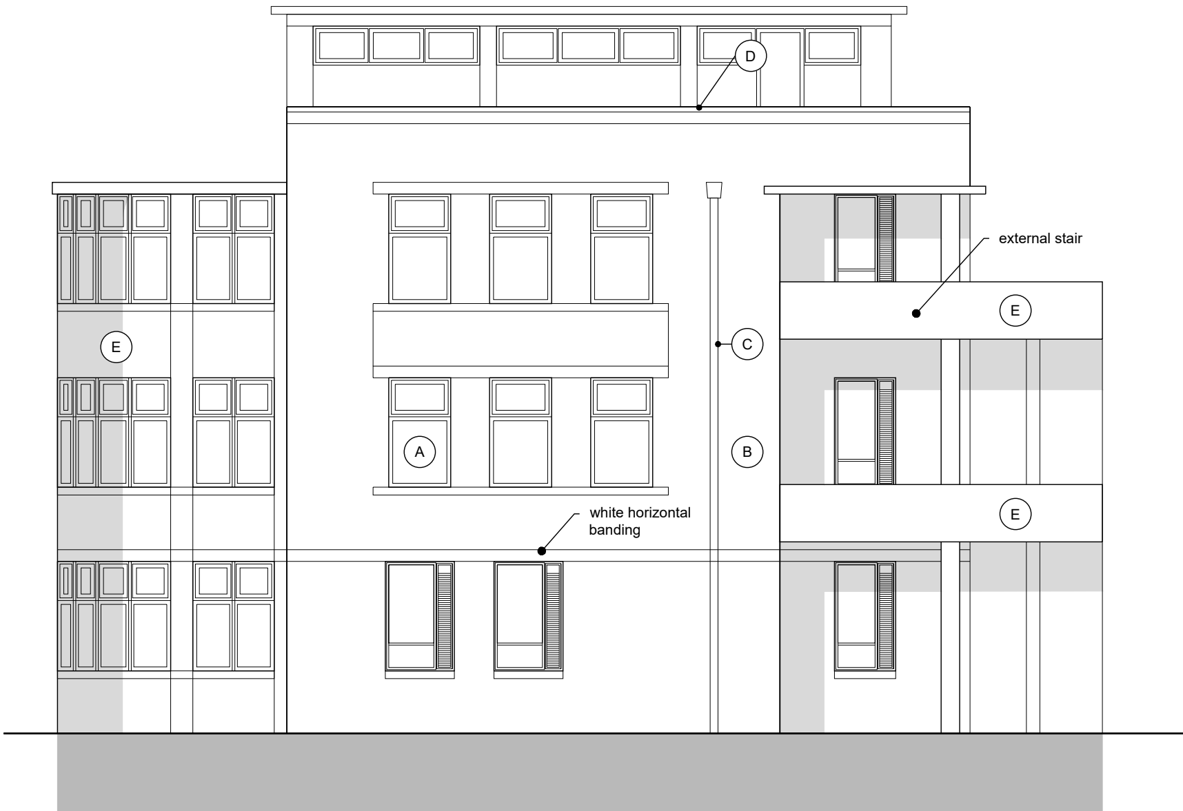
3 Existing - South Elevation
